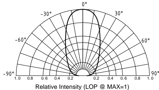
Beam Pattern
