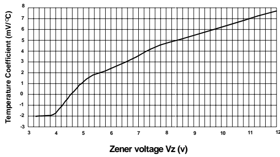
Temperature Coefficient
