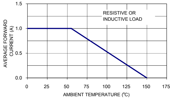
FIG. 1- MAXIMUM AVERAGE FORWARD CURRENT DERATING
