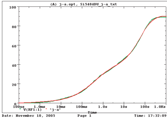
Si5484DU Filter j-a Temperature: 27.0
