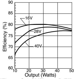
SMFL2805S & SMFL2805D Efficiency
