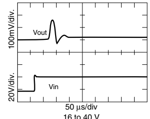
SMFL2805S Step Line Response
