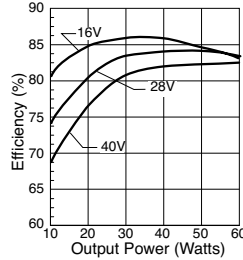
SMFL2812S & SMFL2812D Efficiency
