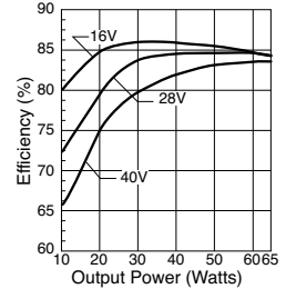
SMFL2815S & SMFL2815D Efficiency
