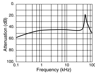
SMFL Series Audio Rejection
