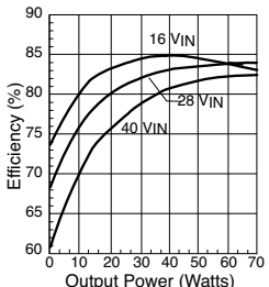
SMFL2828S Efficiency
