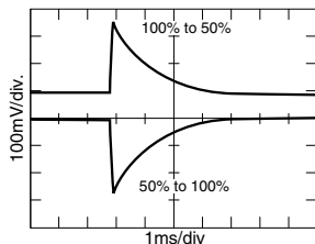
SMFL2805S Step Load Response
