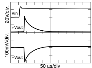
SMFL2815D Step Line Response
