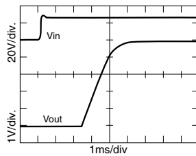
SMFL2805S Turn On Response
