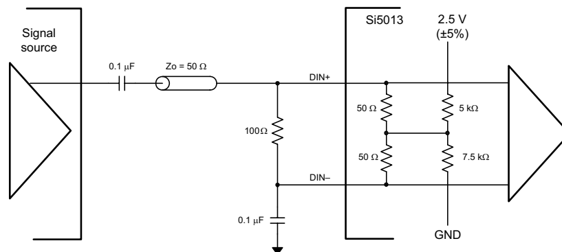
Figure 13. Single-Ended Input Termination for DIN (ac coupled)
