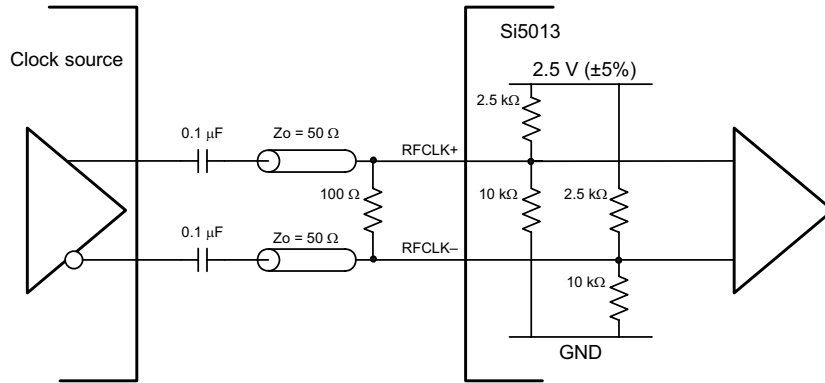
Figure 10. Input Termination for REFCLK (ac coupled)
