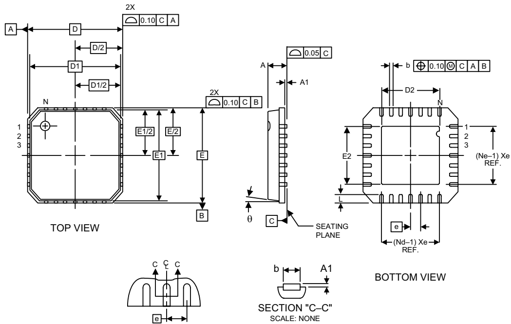
Figure 16. 28-Lead Micro Leaded Package (MLP)
