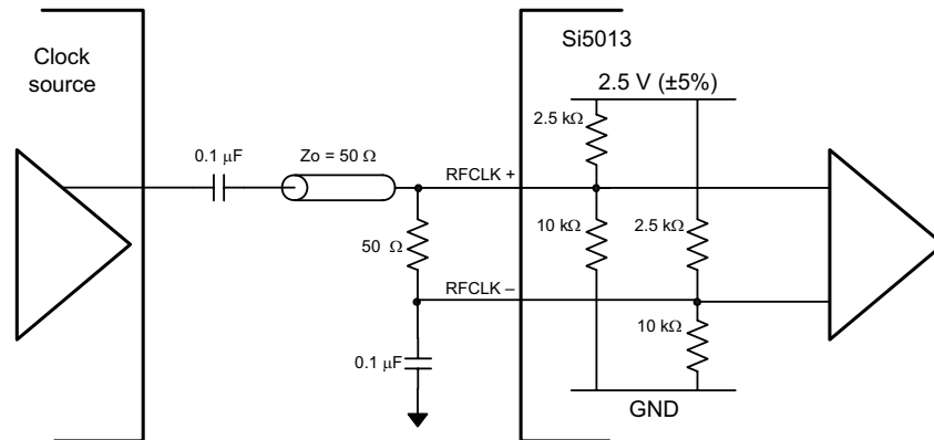
Figure 12. Single-Ended Input Termination for REFCLK (ac coupled)
