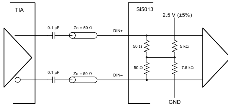
Figure 11. Input Termination for DIN (ac coupled)
