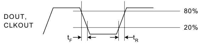
Figure 3. DOUT and CLKOUT Rise/Fall Times
