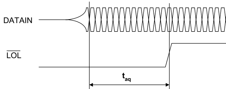
Figure 4. PLL Acquisition Time
