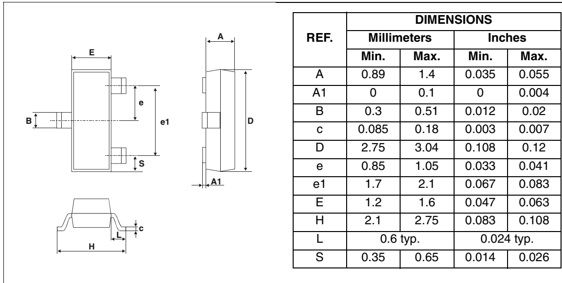
Figure 13: SOT23-3L Package Mechanical Data
