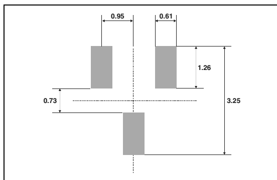
Figure 14: Foot Print Dimensions (in millimeters)
