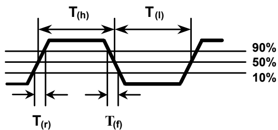
Figure 9. S/PDIF Output
