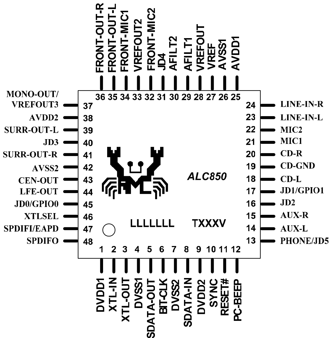
Figure 2. Pin Assignments
