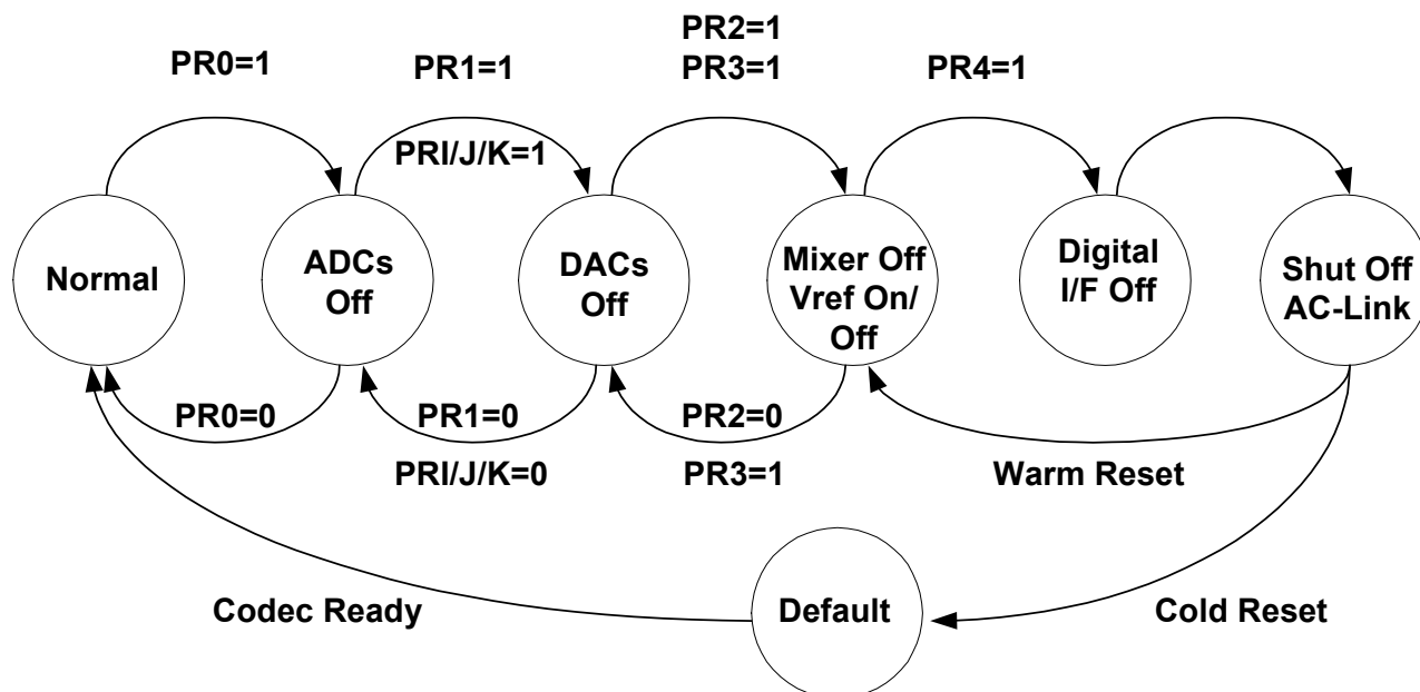
Figure 11. Power-Down Control
