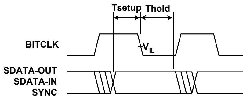
Figure 5. Data Output and Input Timing
