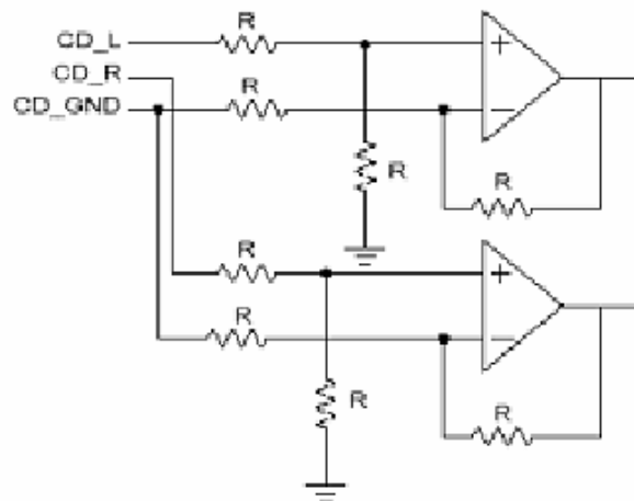
Figure 10. Example of Differential CD Input
