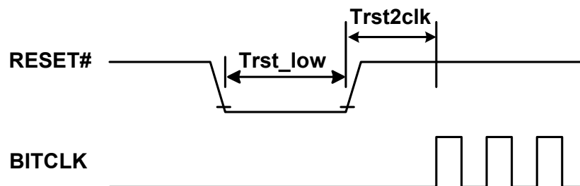
Figure 3. Cold Reset Timing
