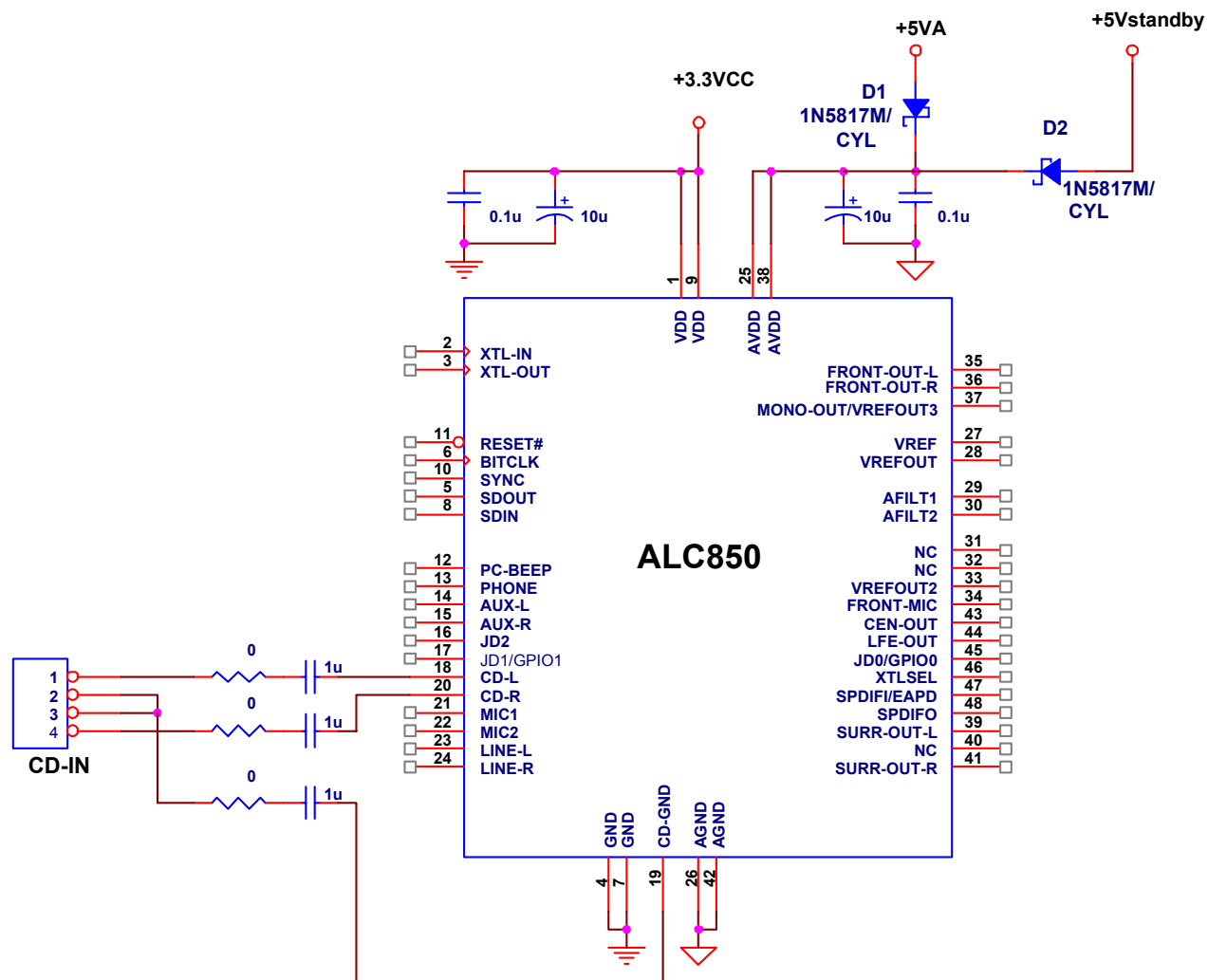
Figure 12. Power-Off CD Function Circuitry
