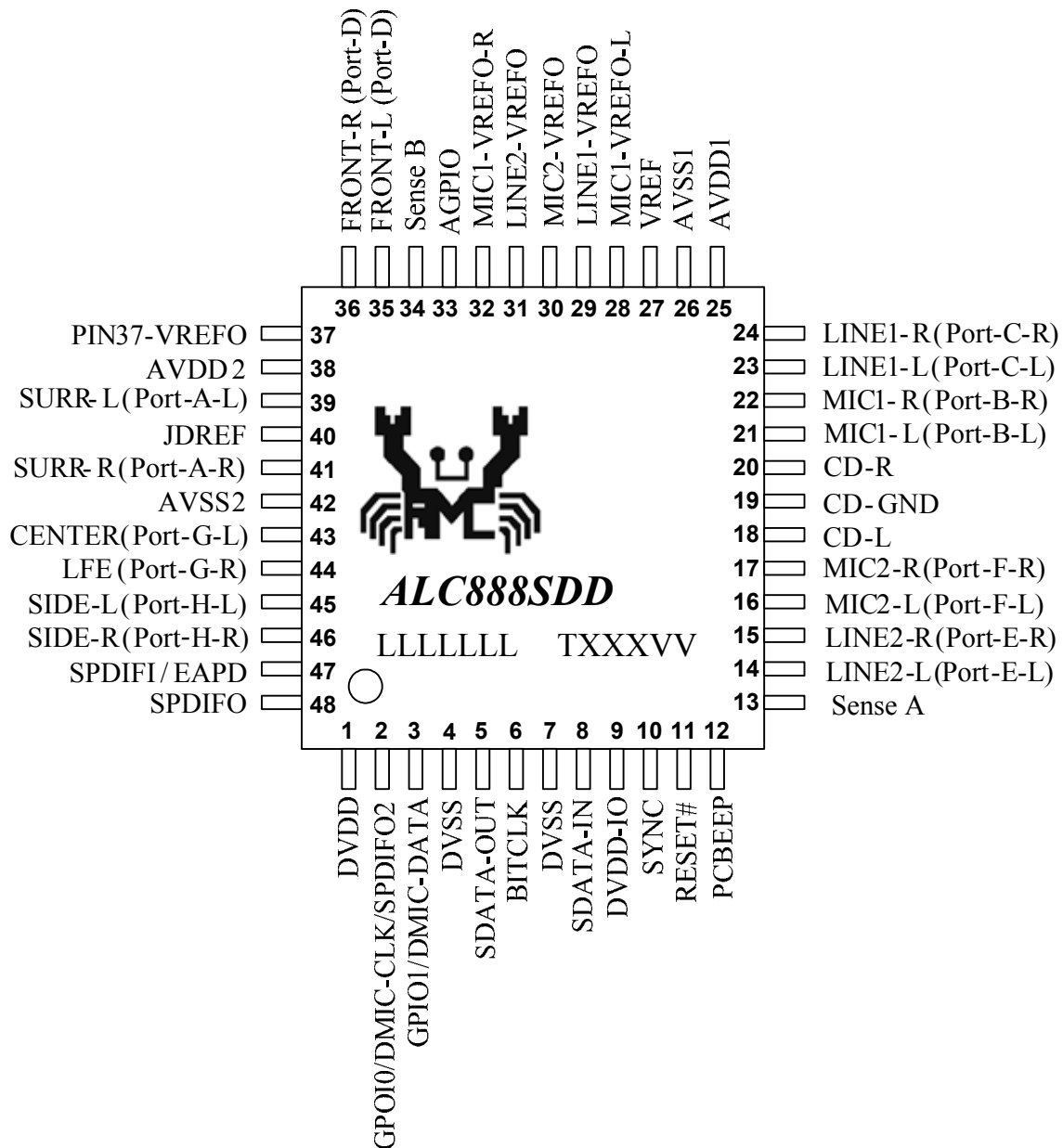
Figure 4. ALC888SDD Pin Assignments
