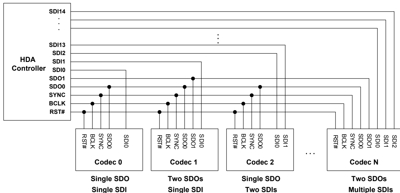
Figure 7. Signaling Topology
