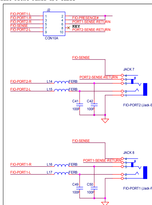
HD Audio Front Panel I/O Cable
