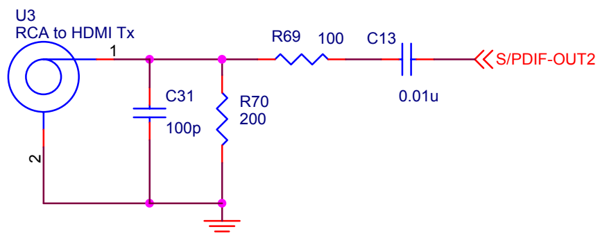
Figure 23. Secondary S/PDIF-OUT Connected to HDMI Tx Connector
