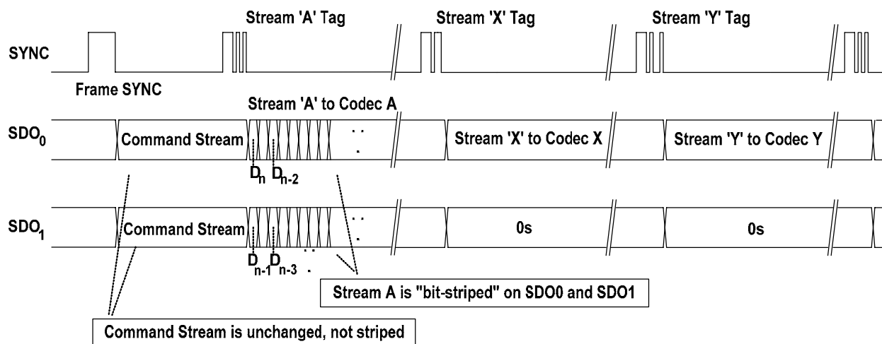
Figure 10. Striped Stream on Multiple SDOs
