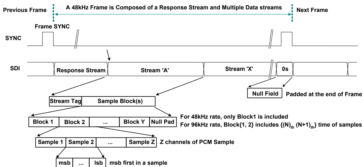
Figure 11. SDI Inbound Stream
