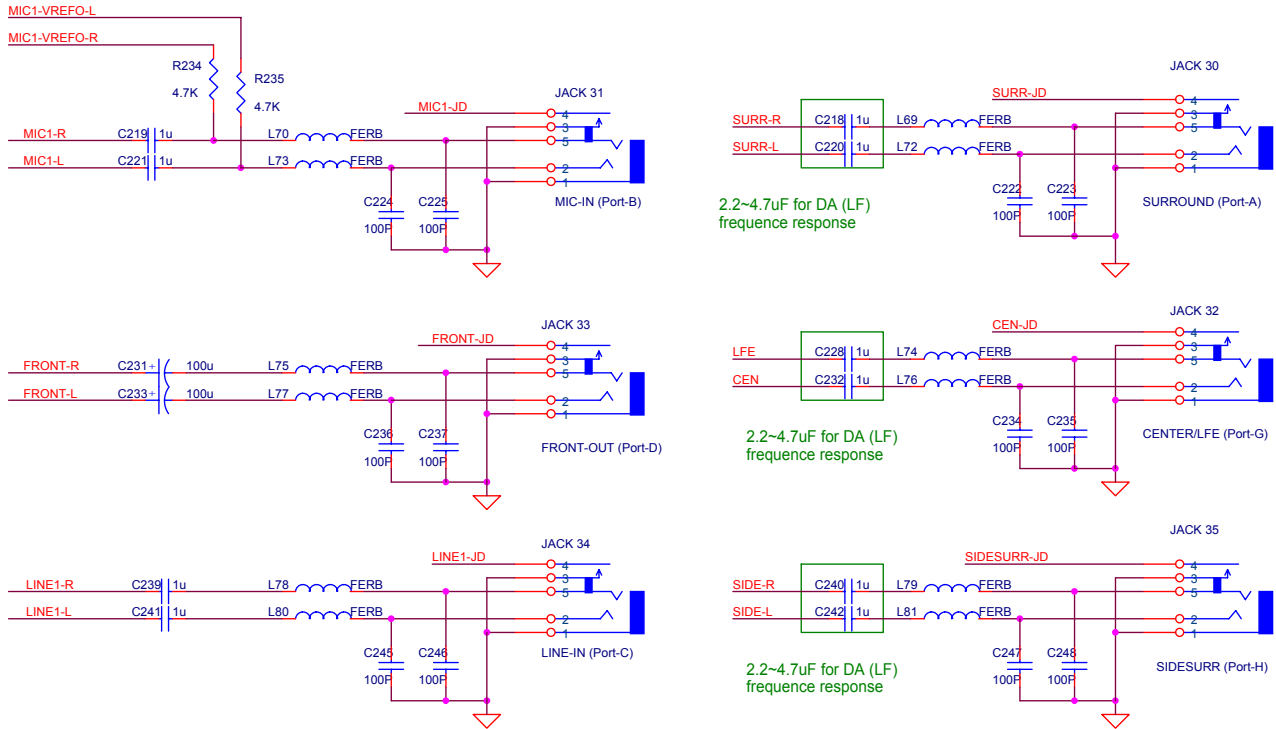
Figure 21. Jack Connection on Rear Panel
