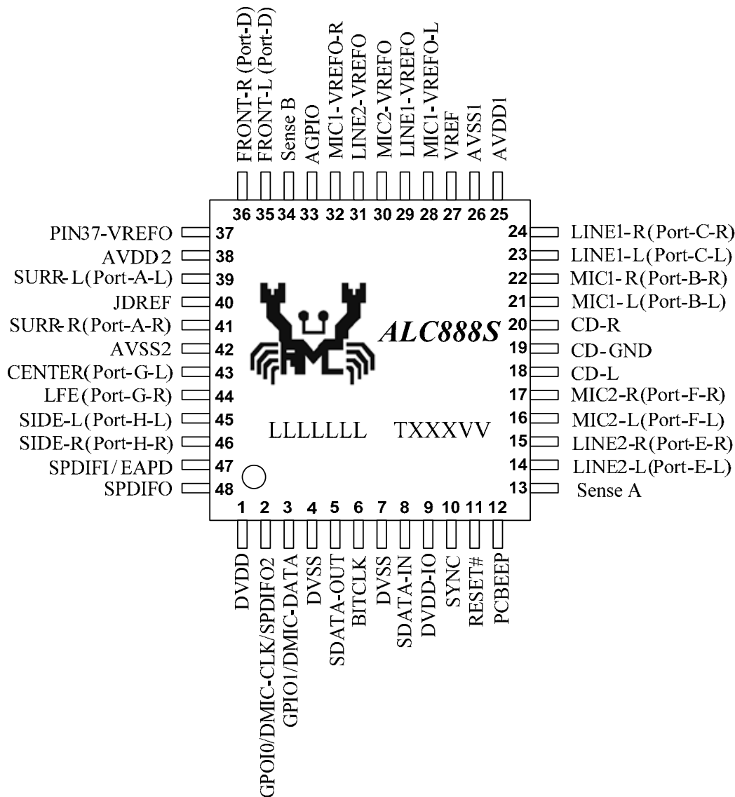
Figure 3. ALC888S Pin Assignments
