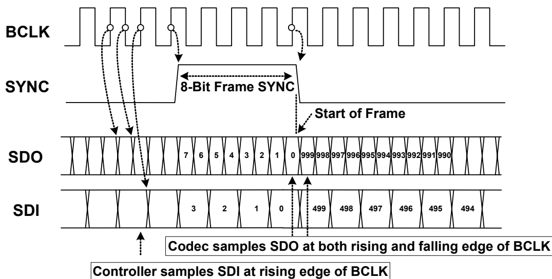
Figure 6. Bit Timing
