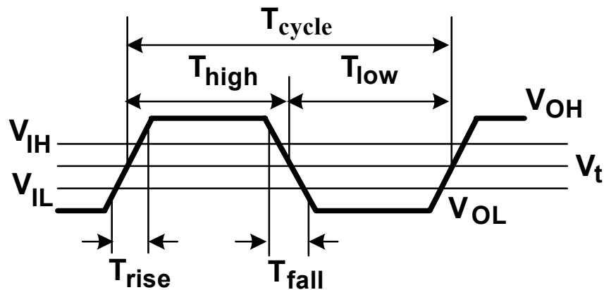
Figure 18. Output and Input Timing
