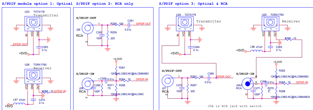
Figure 22. S/PDIF Input/Output Connection
