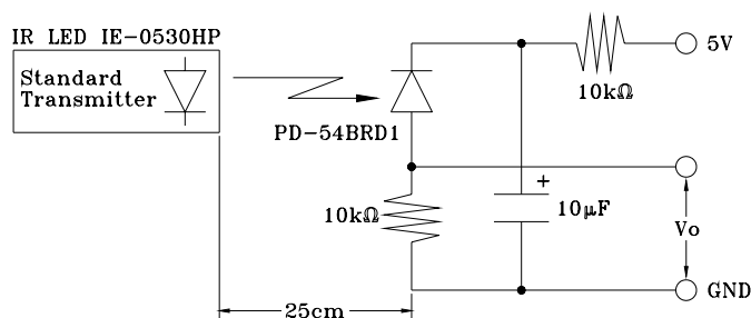
FIG-3 Power Output Measurement Circuit
