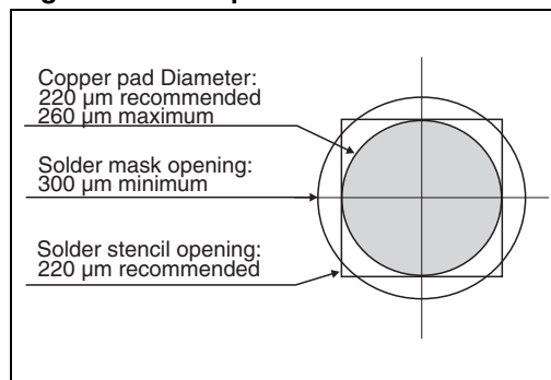
Figure 12. Footprint
