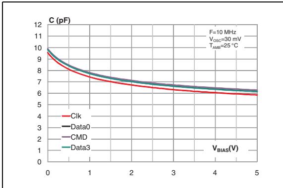
Figure 5. Line capacitance versus applied voltage (typical values)
