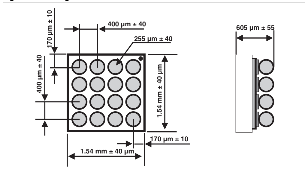
Figure 11. Package dimensions
