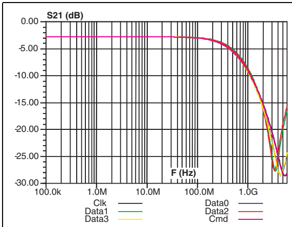
Figure 3. S21 attenuation measurements
