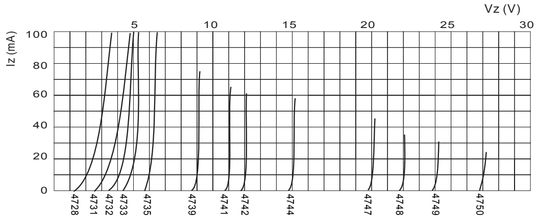
FIG.1 – BREAKDOWN CHARACTERISTICS
