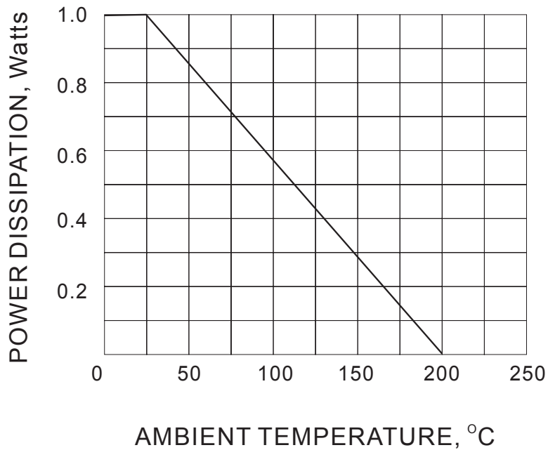
FIG.2 – ADMISSIBLE POWER DISSIPATION VERSUS AMBIENT TEMPERATURE
