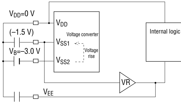
(Figure 4) 3.0 V Operation (Backup Flag="0")
