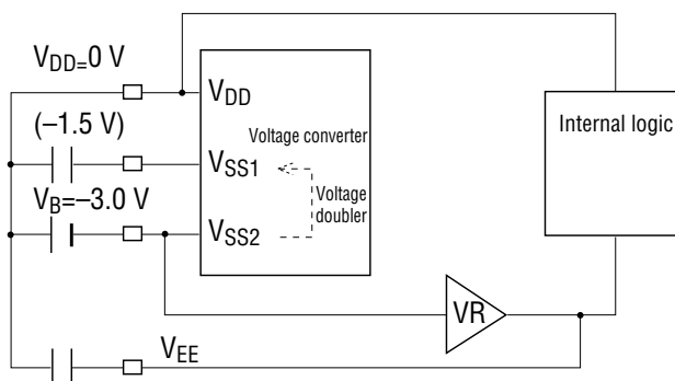
(Figure 3) 3.0 V Operation (Backup Flag="1")
