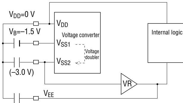
(Figure 2) 1.5 V Operation (Backup Flag="0")
