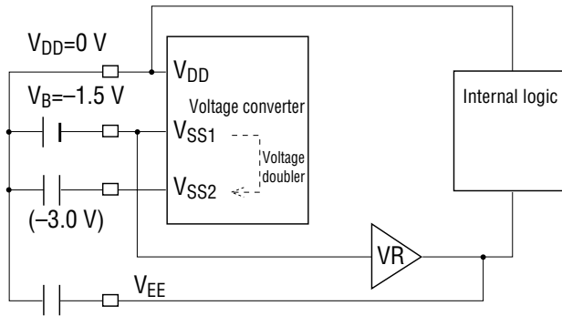
(Figure 1) 1.5 V Operation (Backup Flag="1")
