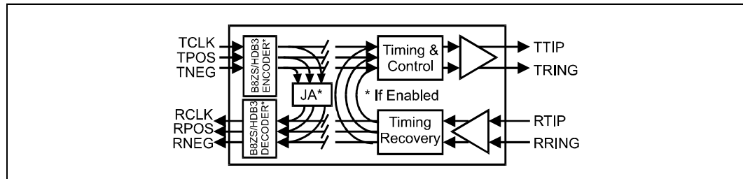
Figure 8. Dual Loopback
