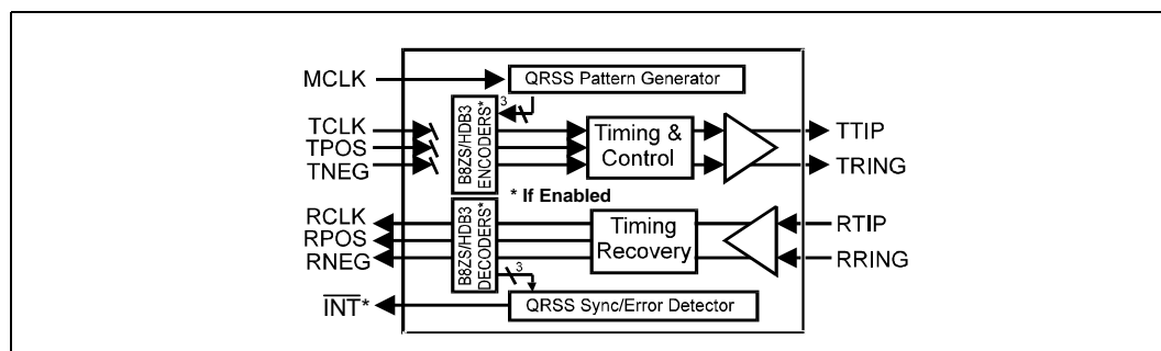
Figure 10. QRSS Mode
