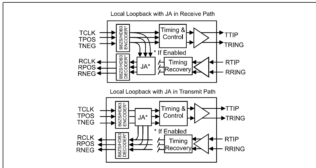
Figure 4. Local Loopback
