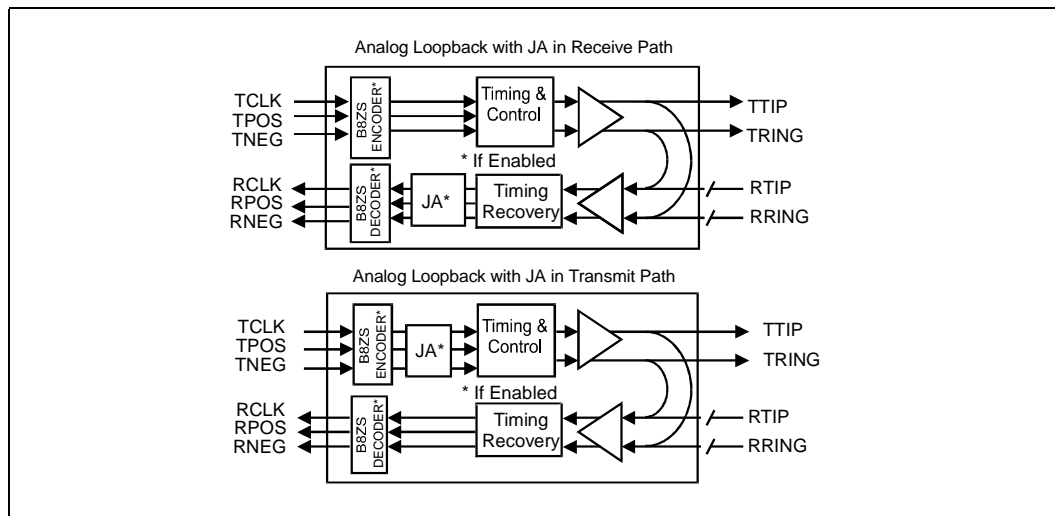
Figure 7. Analog Loopback
