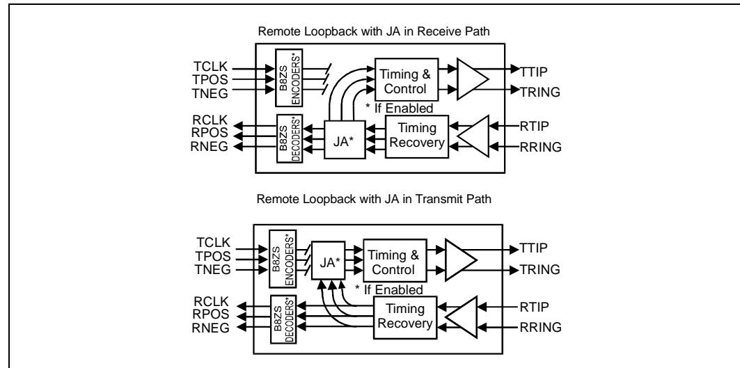
Figure 8. Remote Loopback
