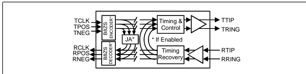
Figure 9. Dual Loopback
