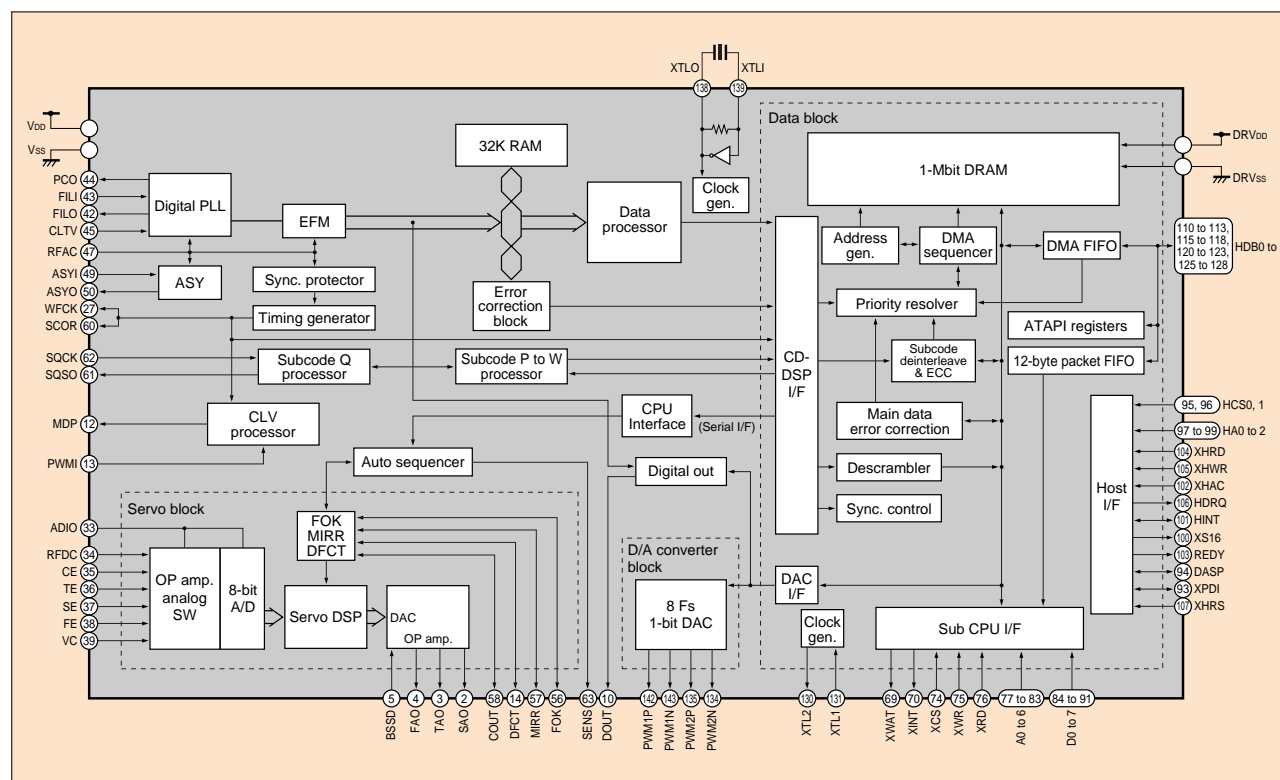
■ Figure 2 CXD3030R Block Diagram
