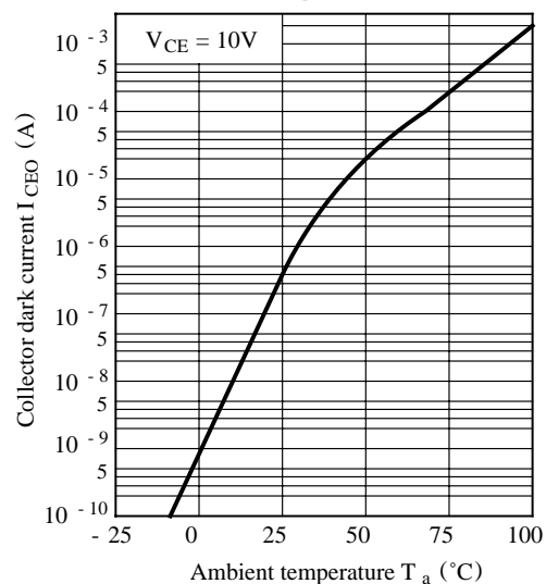
Fig. 9 Collector Dark Current vs. Ambient Temperature
