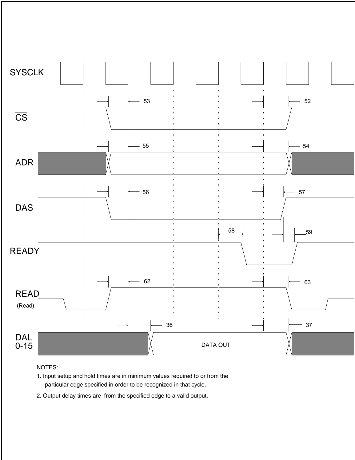
Figure 13: MK50H28 BUS Slave Timing Diagram (Read)
