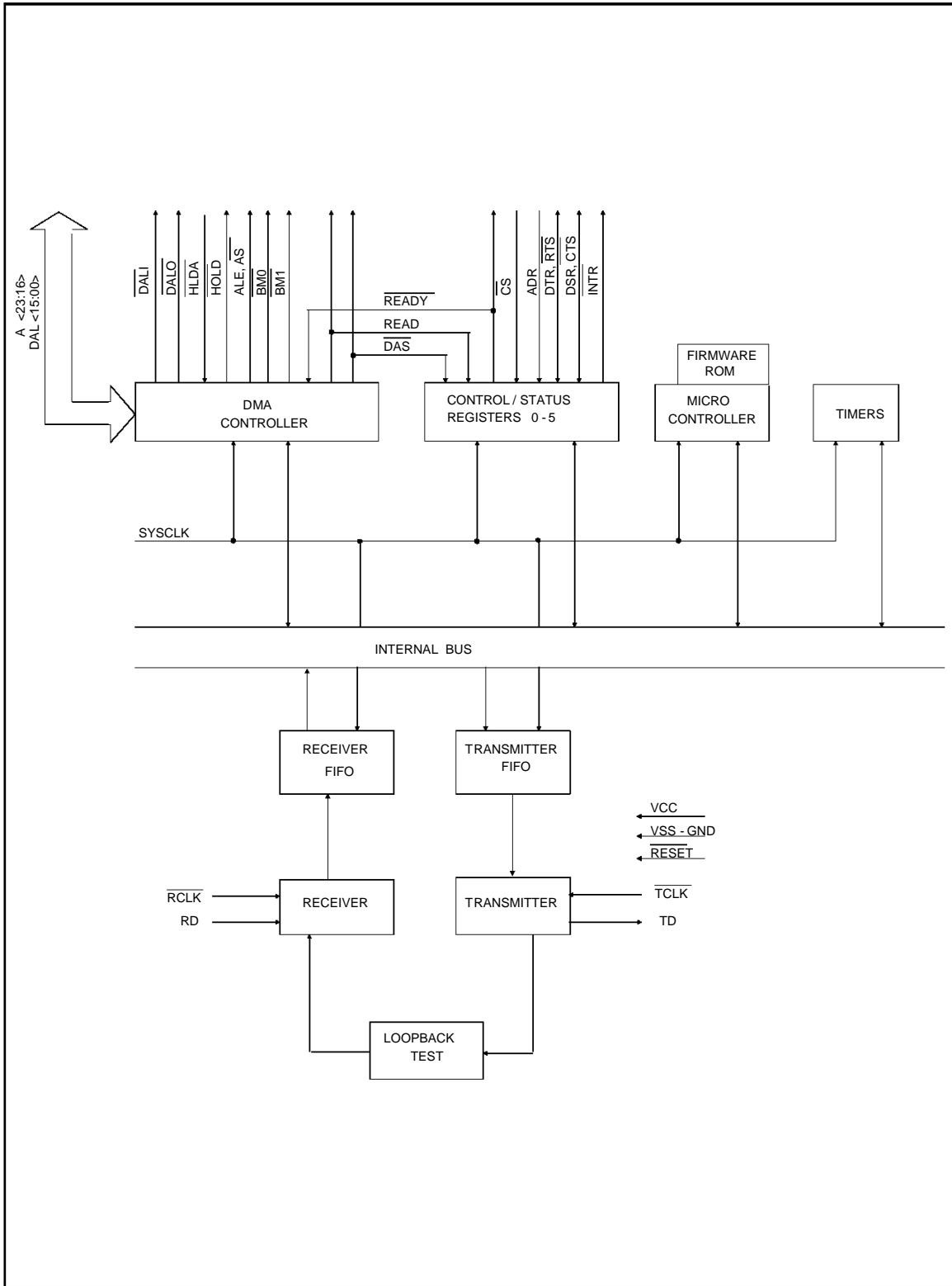
Figure 2: MK50H27 Simplified Block Diagram
