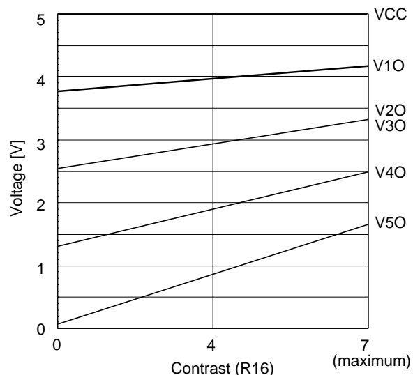
Example 2. LCD bias level Partial Display(1/4 bias,VCC=5V,GND=0V)
