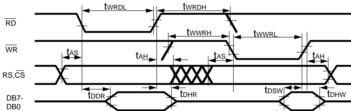
Figure 44 MPU Interface
