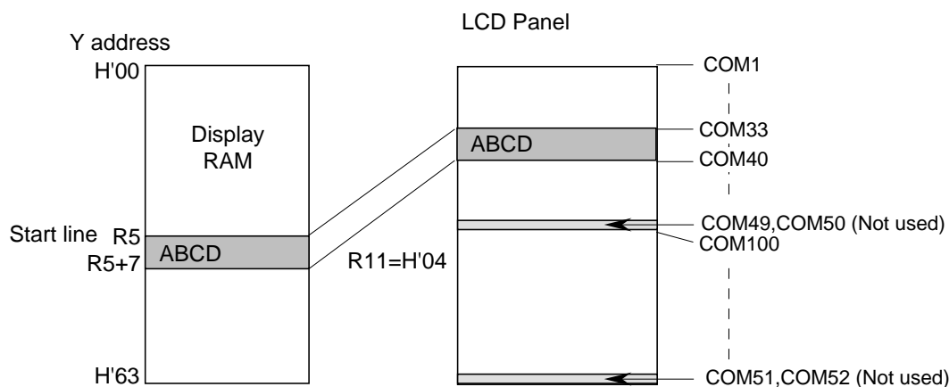
Figure 24 Partial Display
