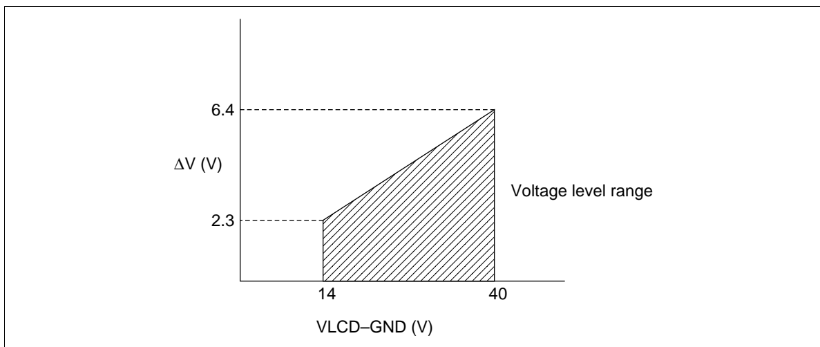
Figure 5 Relation between VLCD–GND and \Delta V
