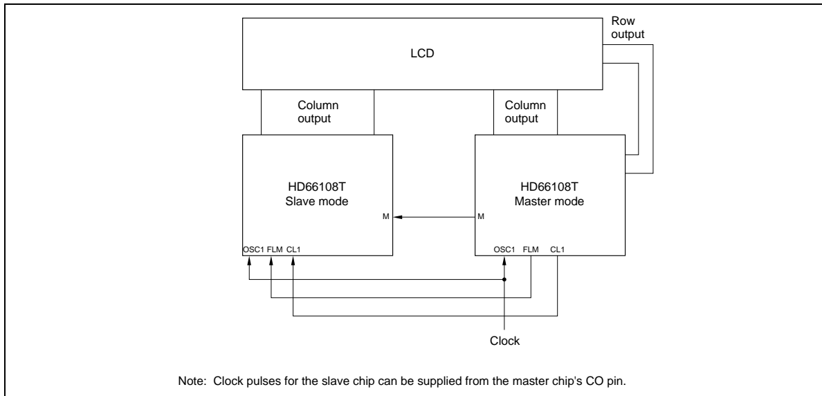
Figure 24 Configuration Using Two HD66108T Chips (1)
