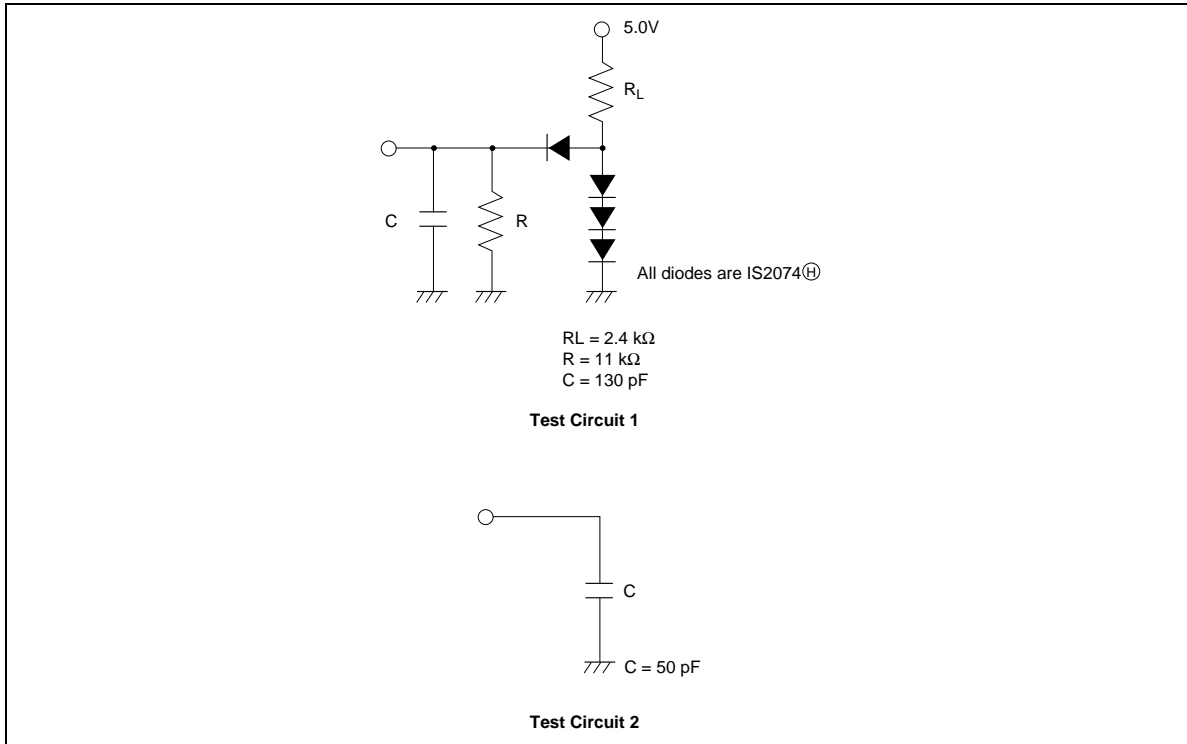
Figure 39 Load Circuits
