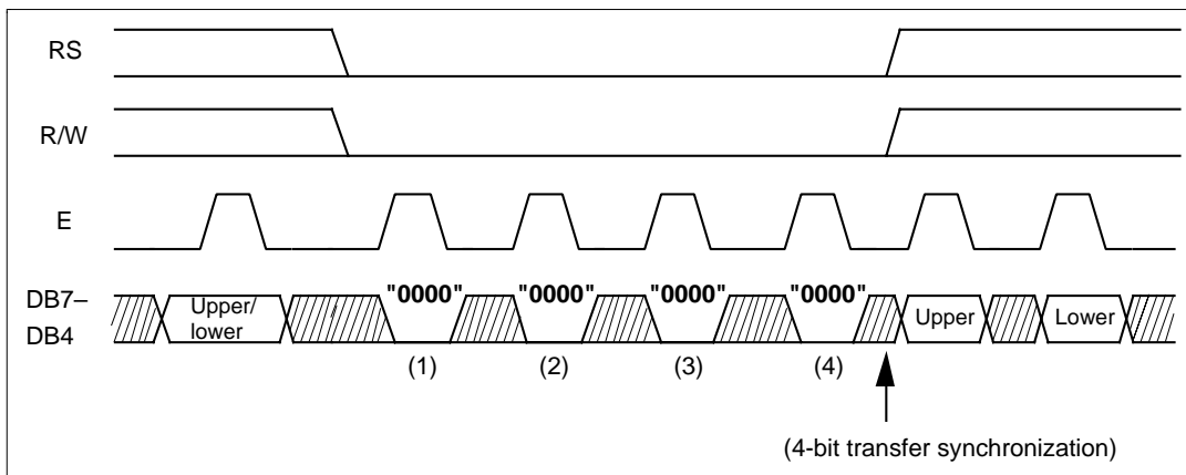
Figure 18 4-bit Transfer Synchronization
