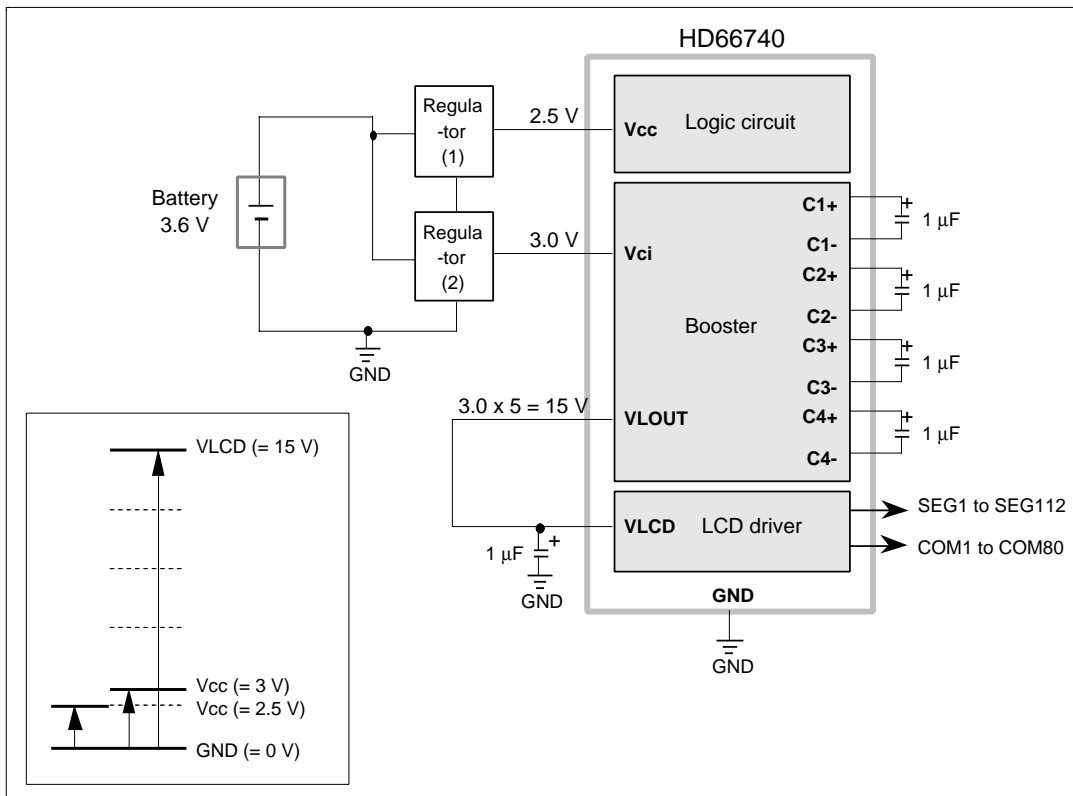
Figure 26 Usage Example of Booster at Vci > Vcc
