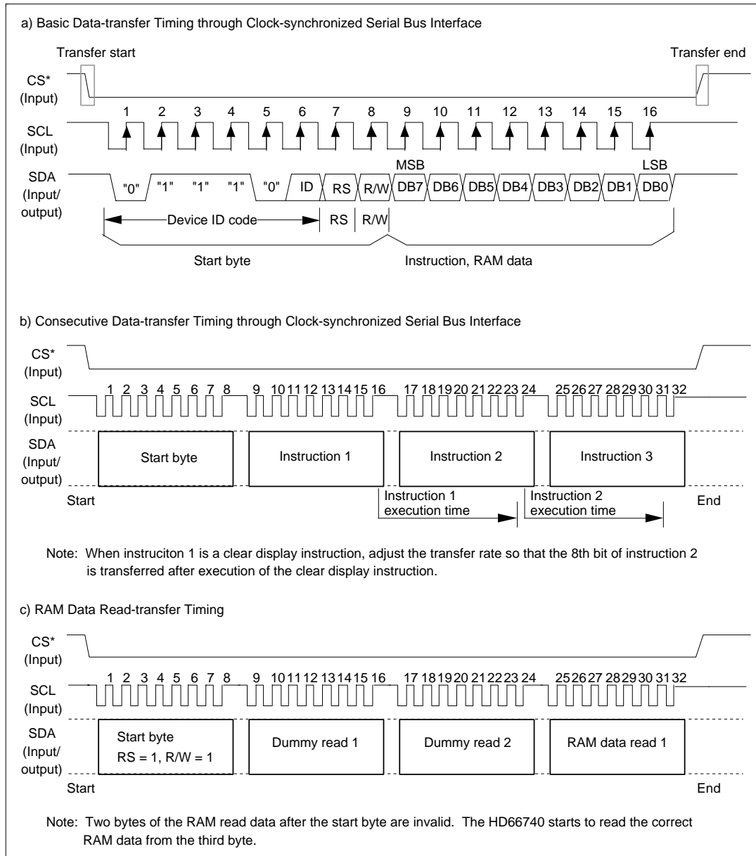
Figure 16 Clock-synchronized Serial Interface Timing Sequence
