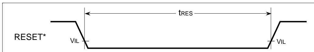
Figure 50 Reset Timing
