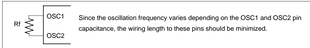
Figure 44 Internal Oscillation
