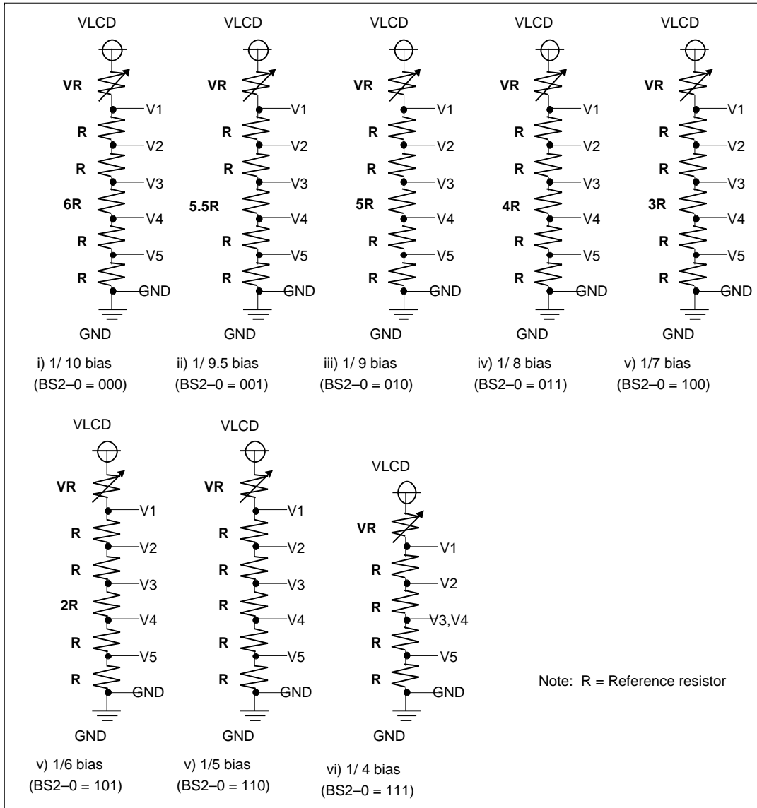
Figure 28 Liquid Crystal Display Drive Bias Circuit
