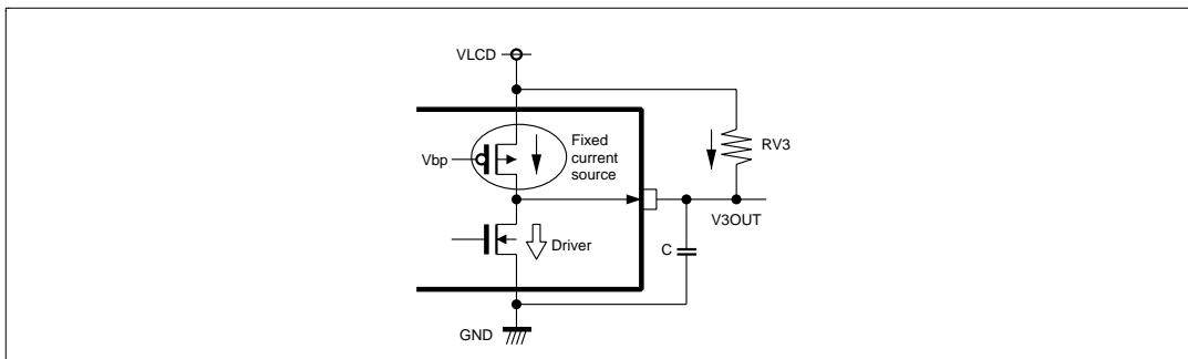
Figure 24-c Countermeasure for V3OUT Output
