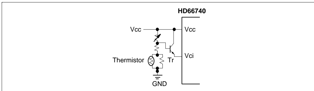
Figure 24 Temperature Compensation Circuit
