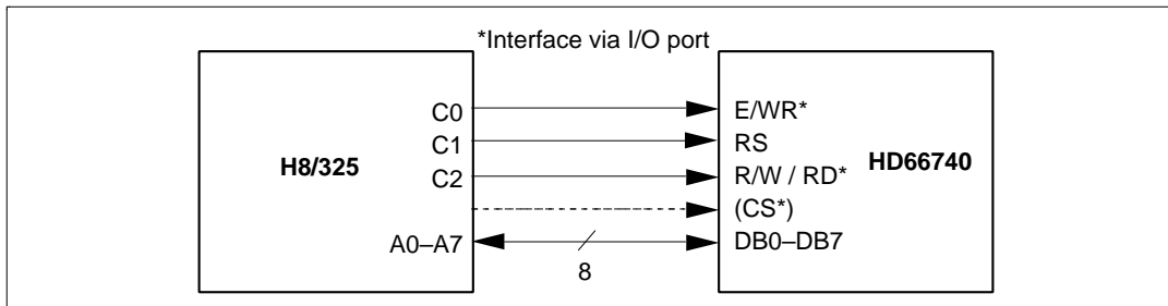
Figure 17 Interface to 8-bit Microcomputer
