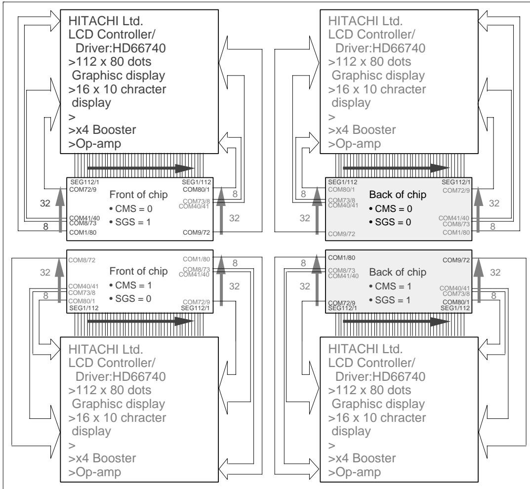
Figure 29 1/80 Duty Drive Pattern Wiring
