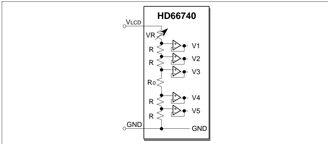
Figure 5 Contrast Adjuster
