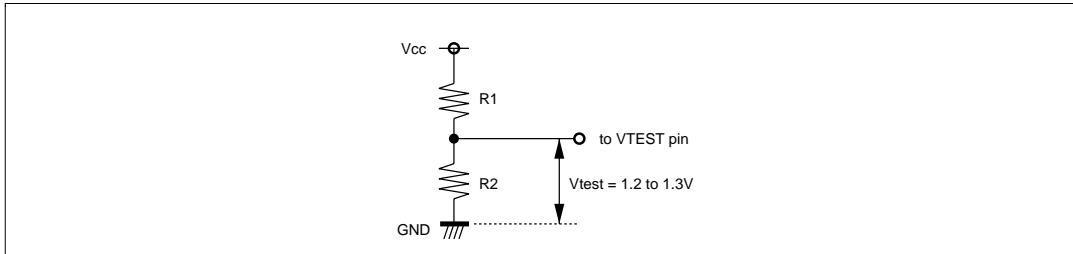
Figure 24-a Circuit to for Generating VTEST Pin Voltage
