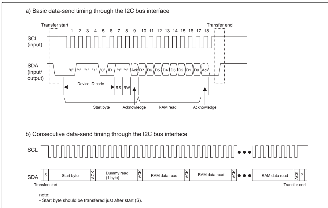
Figure 16-b I2C bus interface data-send sequence
