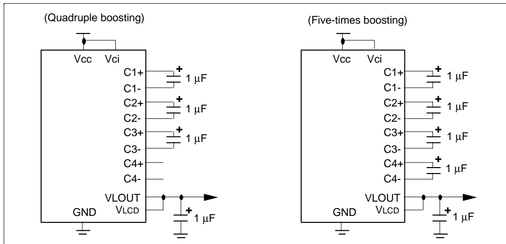
Figure 45 Booster
