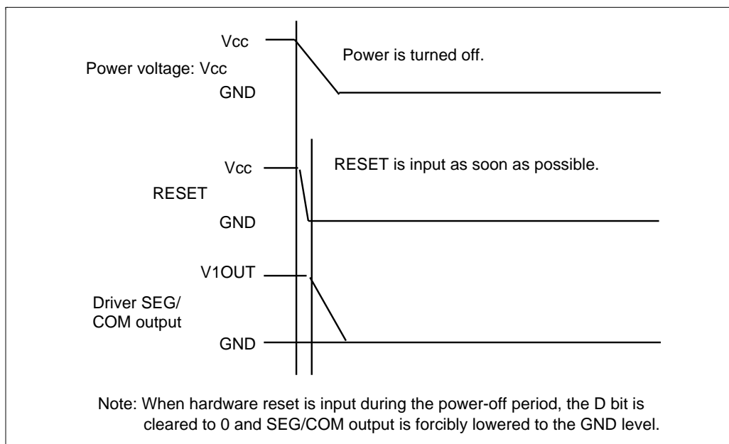
Figure 55 Power-off Timing
