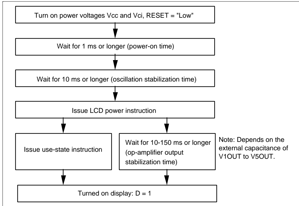
Figure 52 Power-on Sequence
