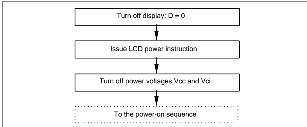
Figure 54 Power-off Sequence
