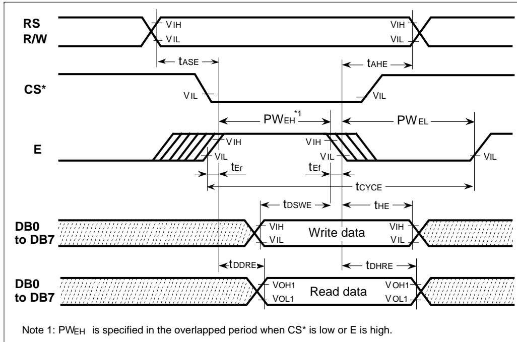
Figure 47 68-system Bus Timing
