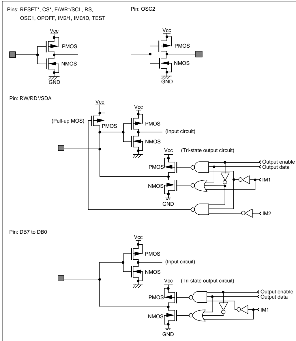
Figure 41 I/O Pin Configuration
