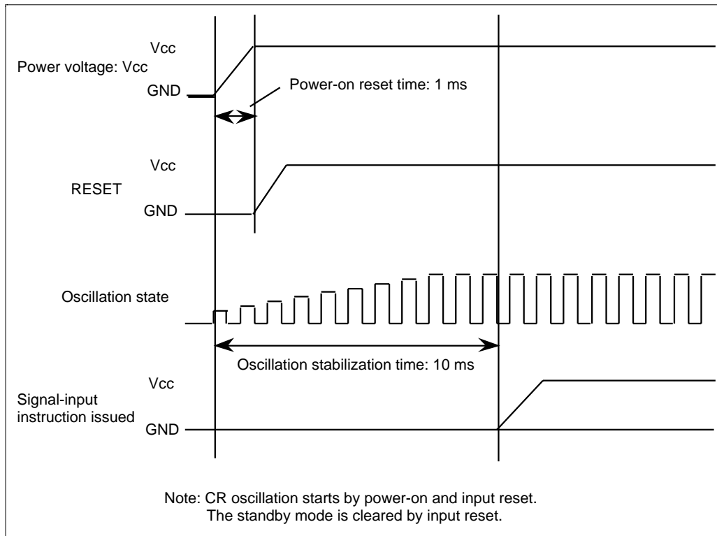
Figure 53 Power-on Timing
