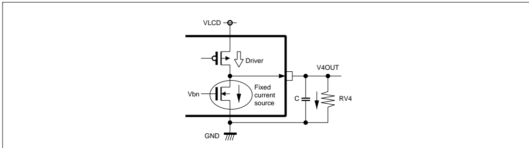
Figure 24-b Countermeasure for V4OUT Output
