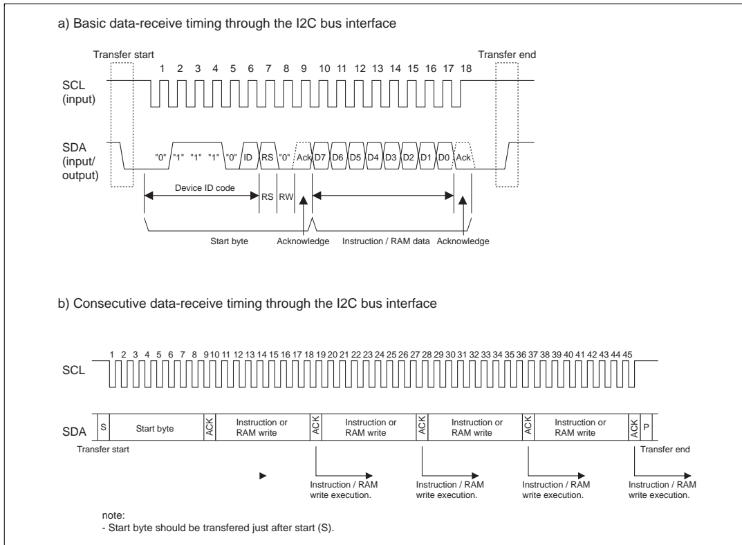
Figure 16-a I2C bus interface data-receive sequence
