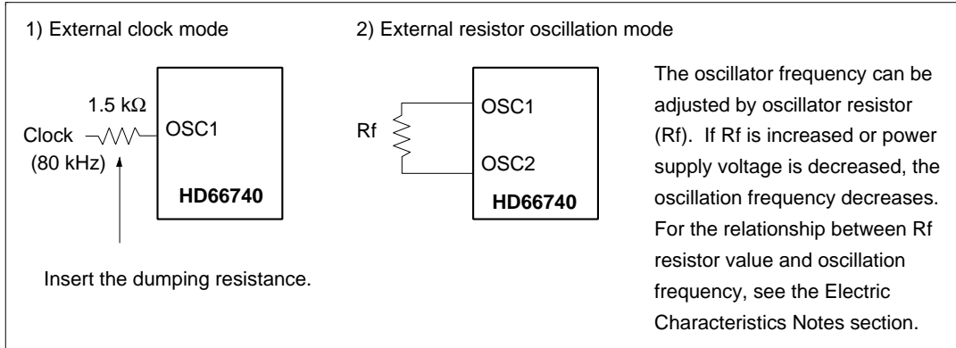
Figure 19 Oscillation Circuits
