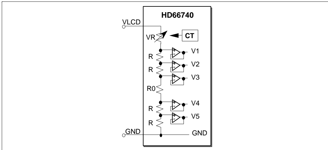
Figure 27 Contrast Adjuster
