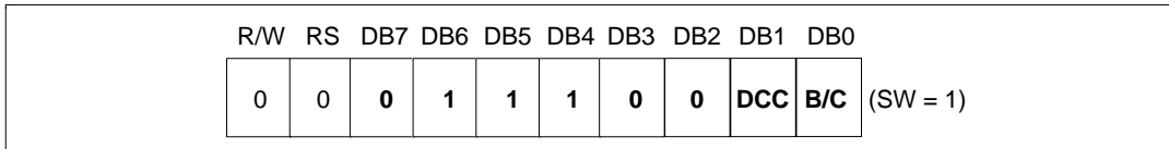
Figure 10a LCD-Driving-Waveform Control Instruction
