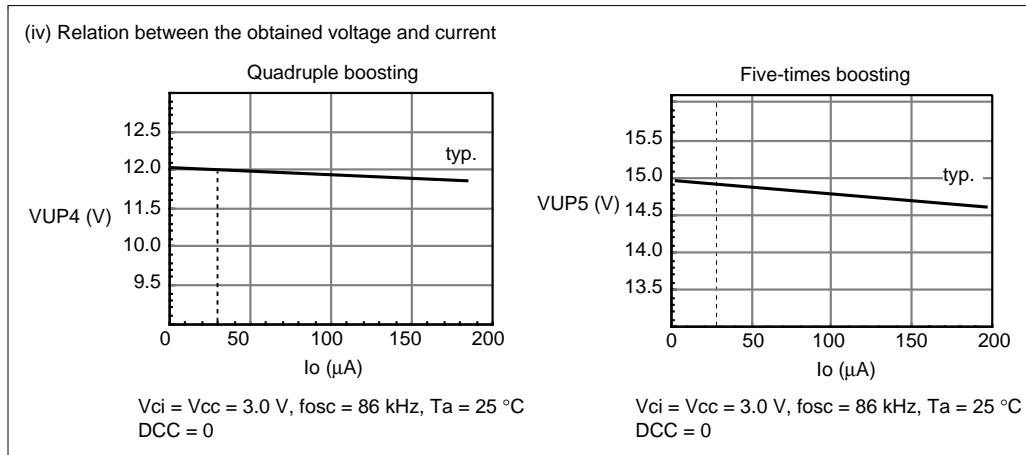
Figure 45 Booster (cont)
