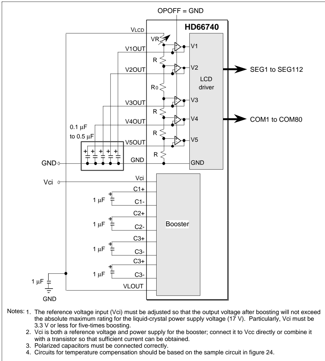
Figure 23 Internal Booster for LCD Drive Voltage Generation
