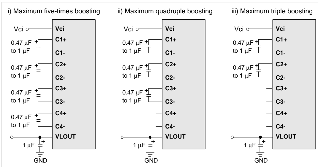
Figure 25 Booster Output Multiplying Factor Switching
