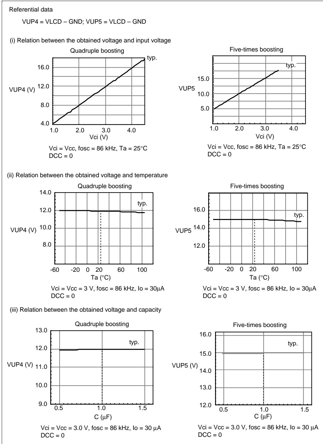
Figure 45 Booster (cont)
