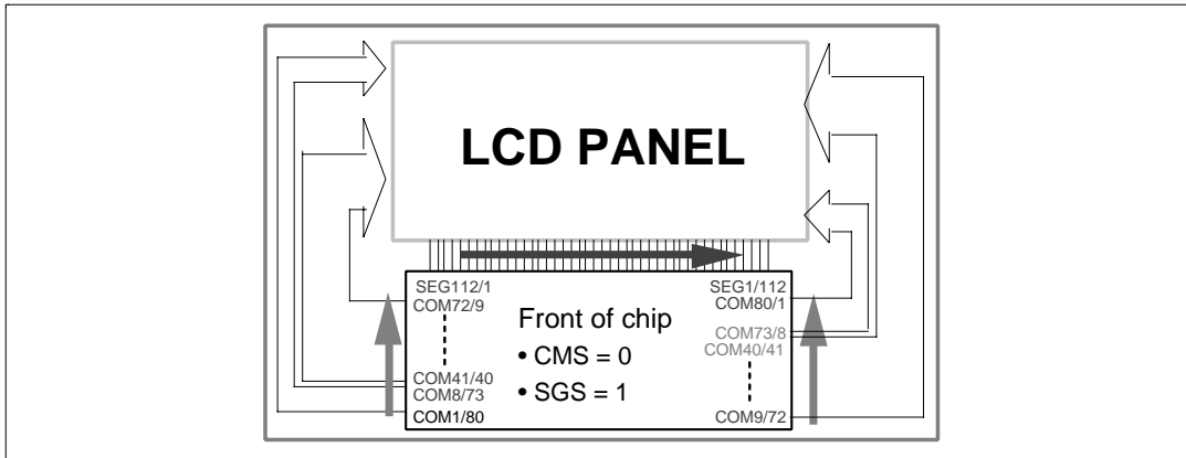
Figure 30 1-line Display Pattern Wiring
