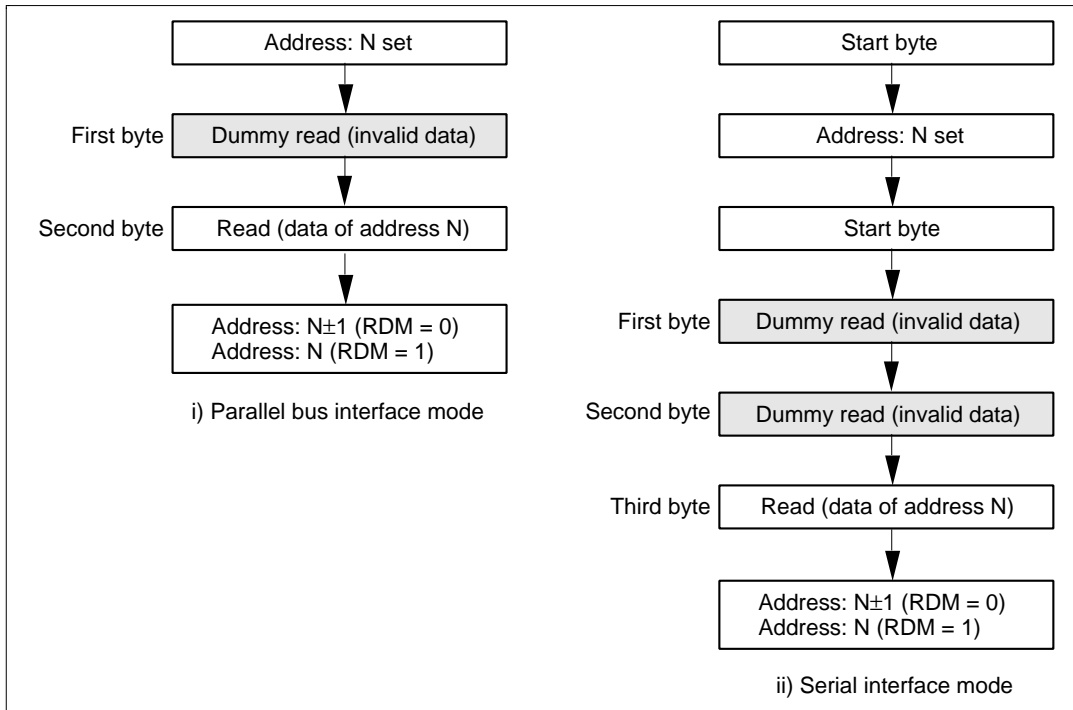
Figure 15 RAM Read Sequence
