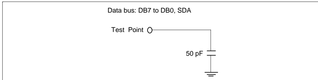
Figure 46 Load Circuit
