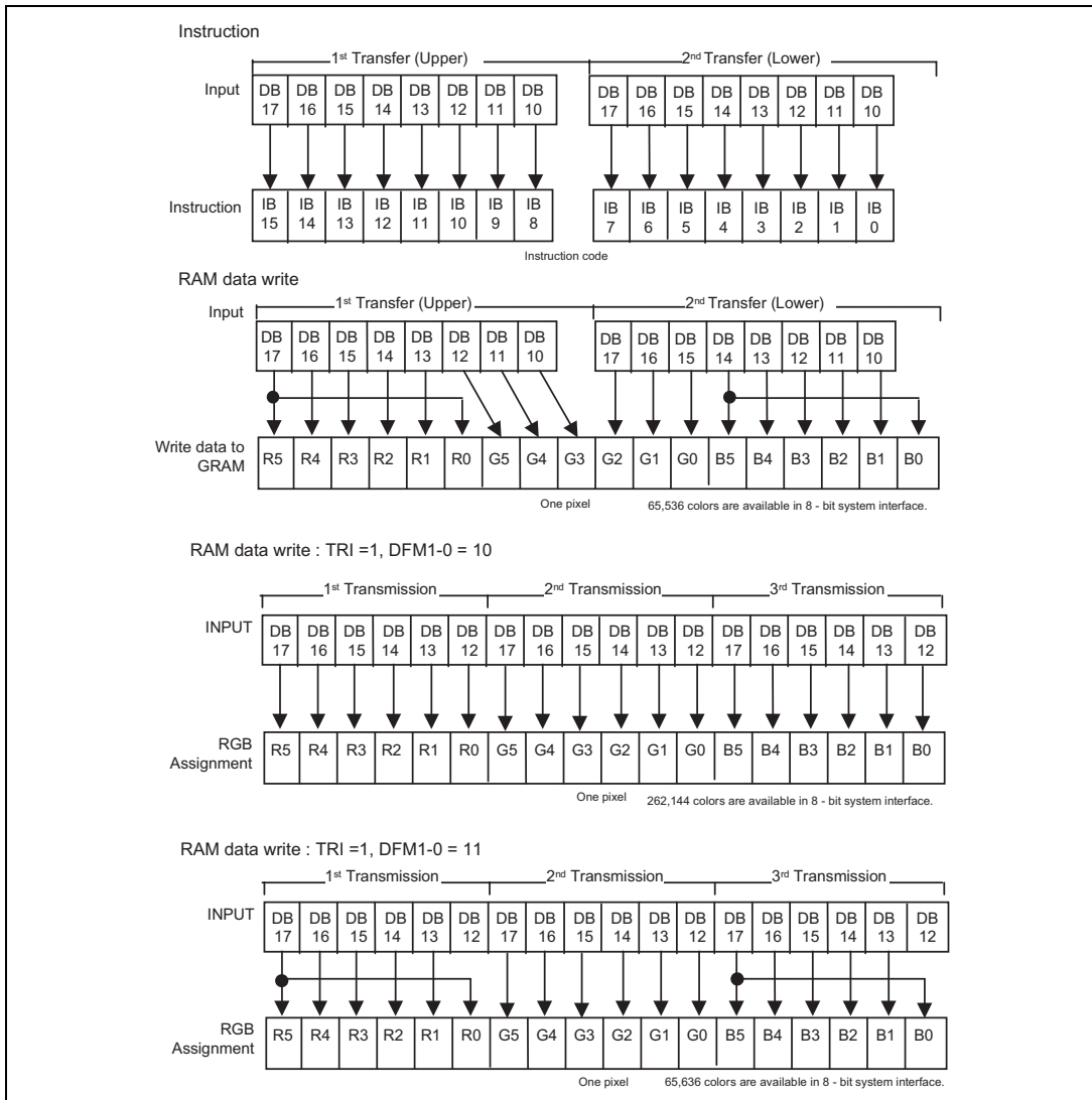
Data format for 8-bit interface
