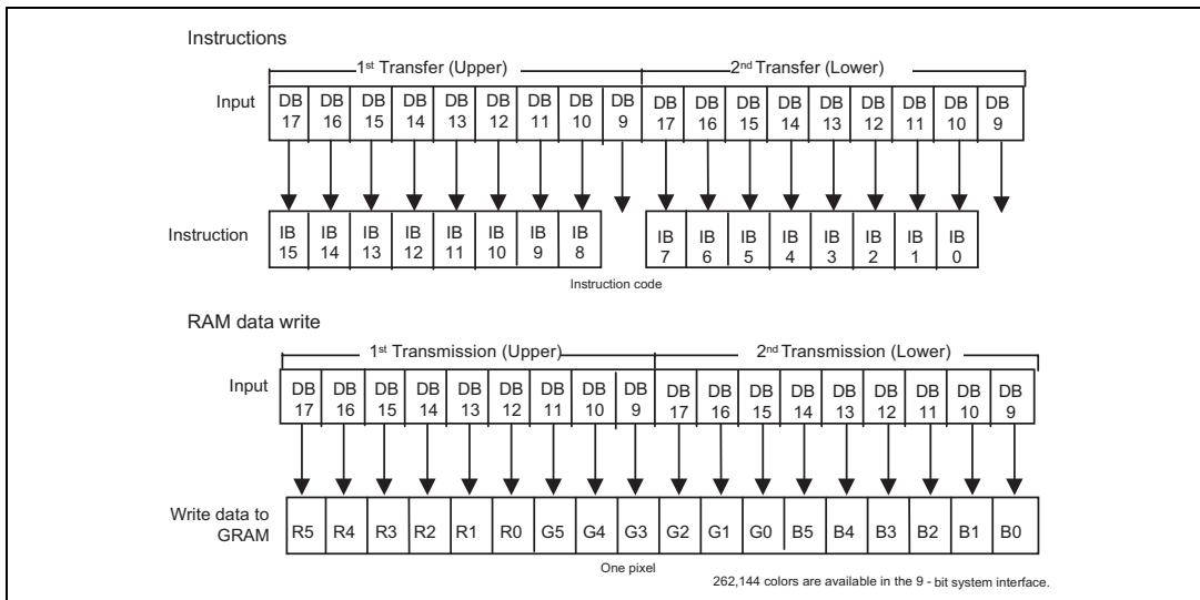
Data format for 9-bit interface
