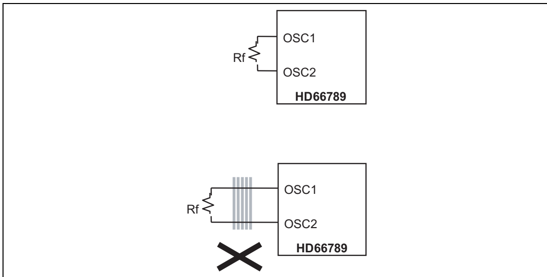
External Resistor Oscillation Mode
