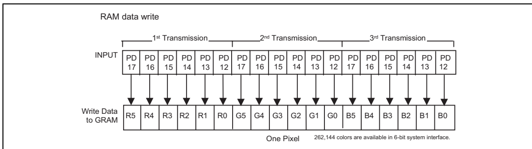
Data format for 6-bit interface
