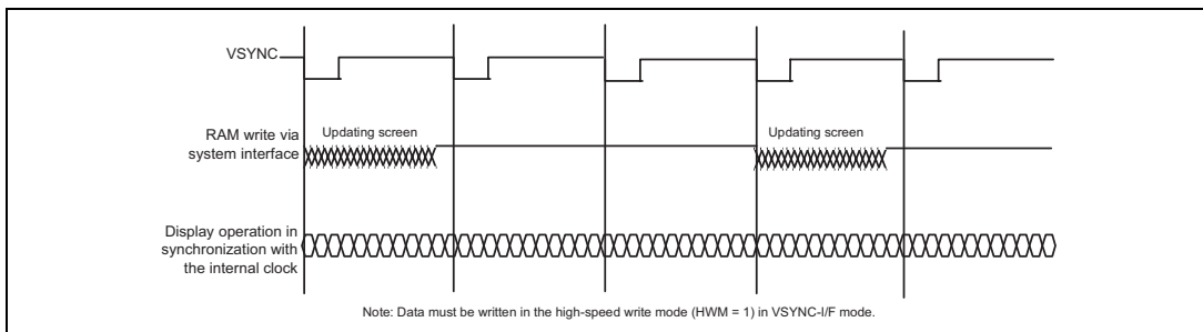
Moving picture data transmission through VSYNC interface
