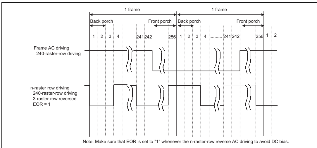
n-raster-rows inversion AC drive
