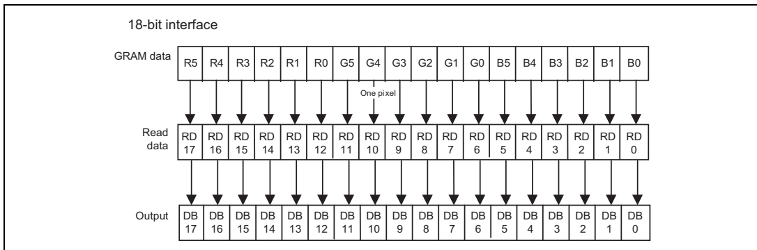
Read data from GRAM: Bit assignment
