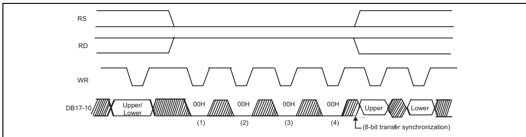
8-bit data transmission synchronization
