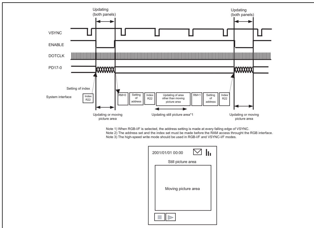
Updating Still Picture Area during Displaying a Moving Picture
