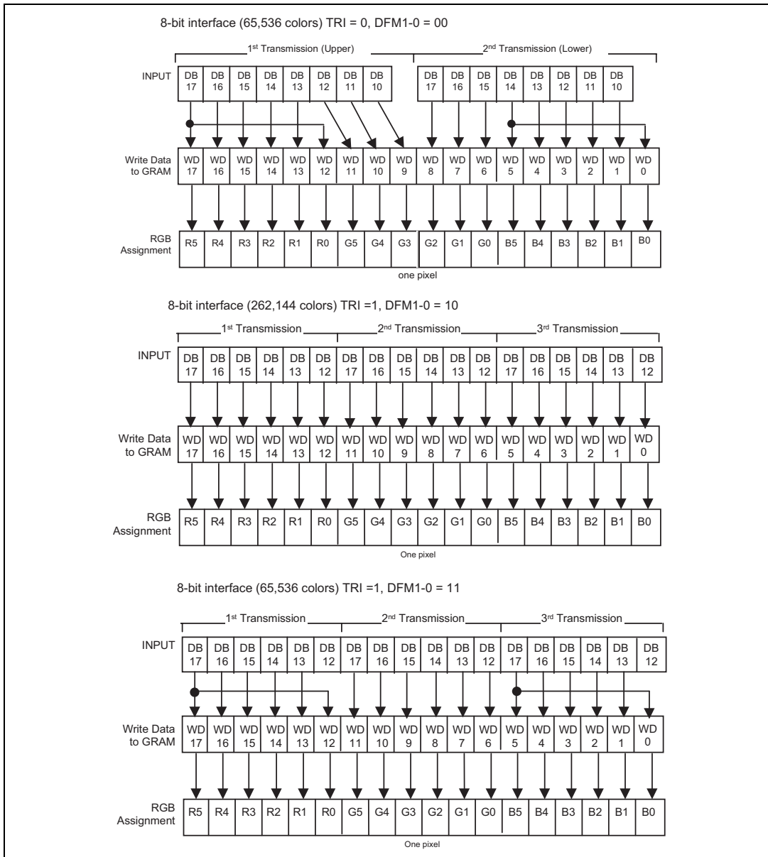
Write data to GRAM: Bit assignment
