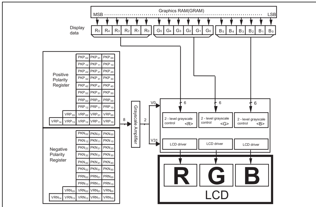
Grayscale control
