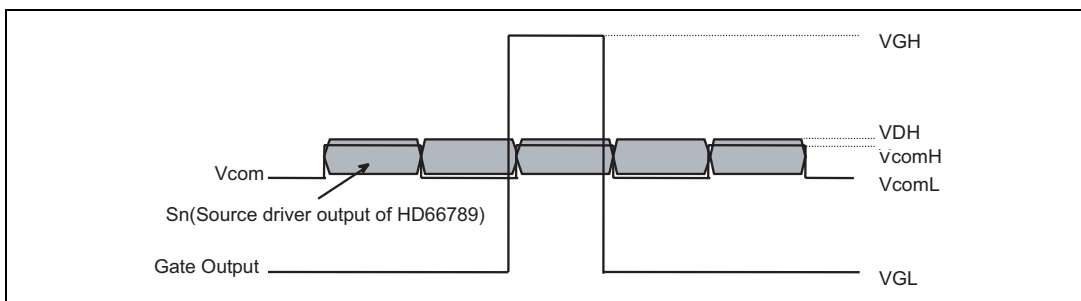
Applied voltage to the TFT display
