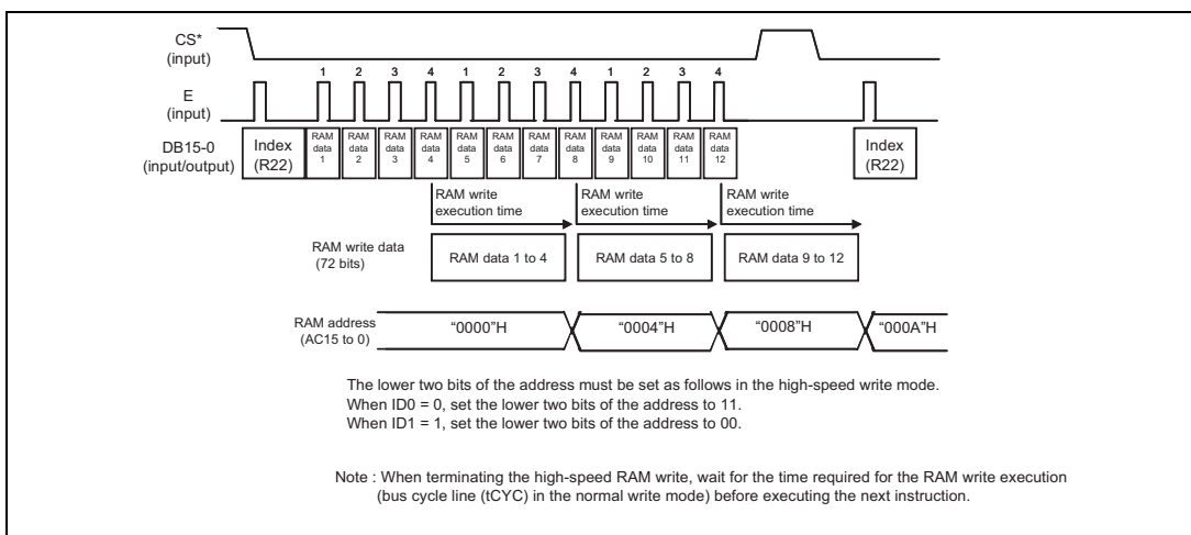
Operational flow of High-Speed Burst RAM Write
