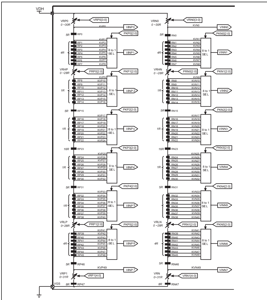
Ladder Resistors and 8-to-1 Selector
