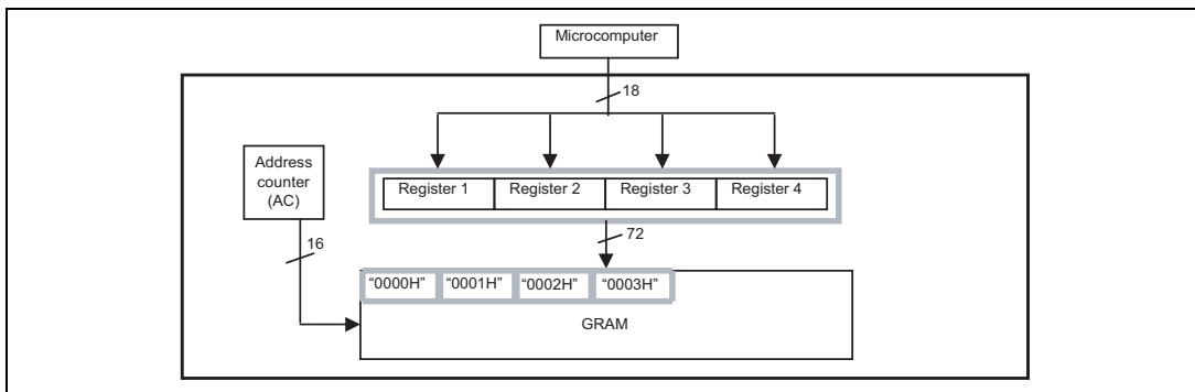
Operational flow of High-Speed Burst RAM Write
