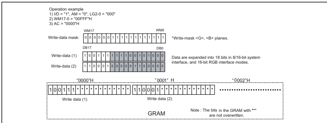
Write Mode 1
