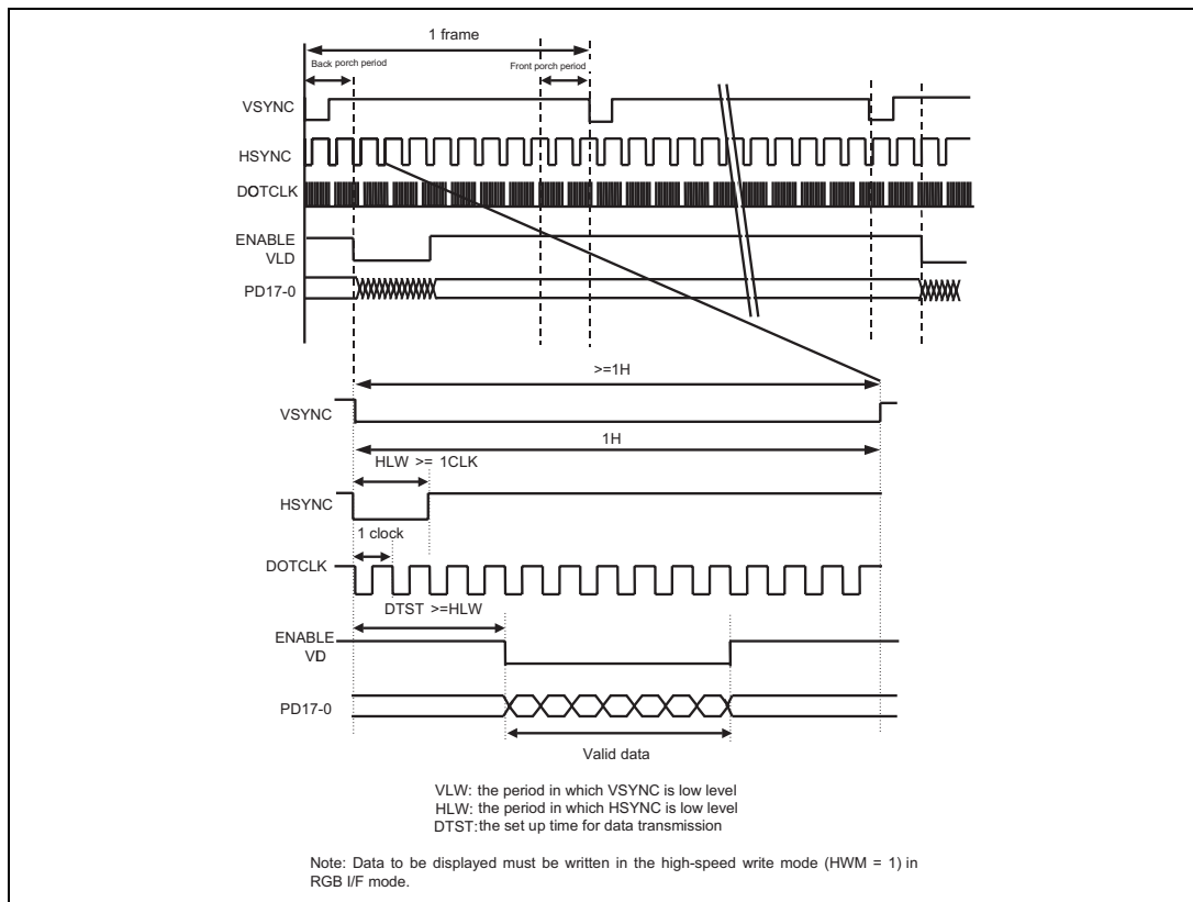
16-/18-bit RGB Interface Timing
