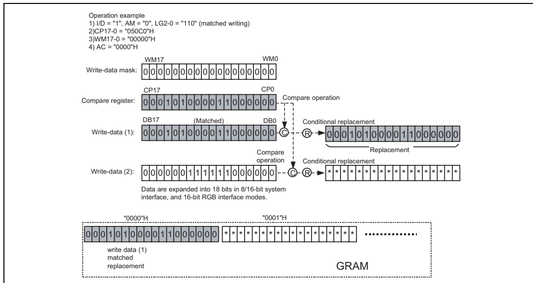
Write Mode 3
