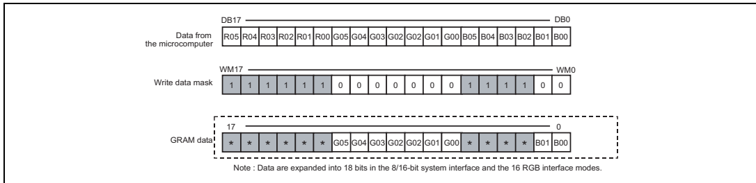
Write data mask function
