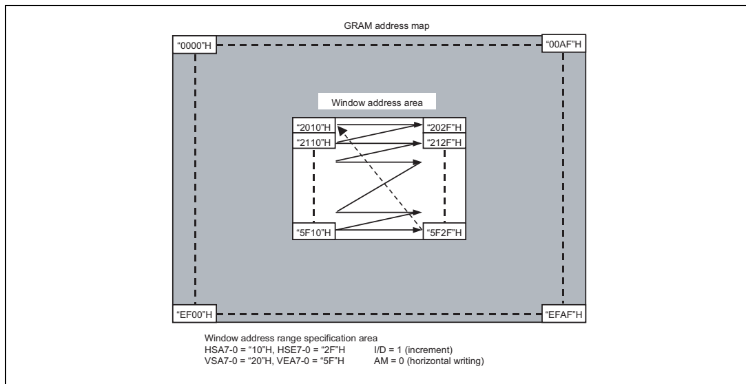
Address transition direction in specified window-address range
