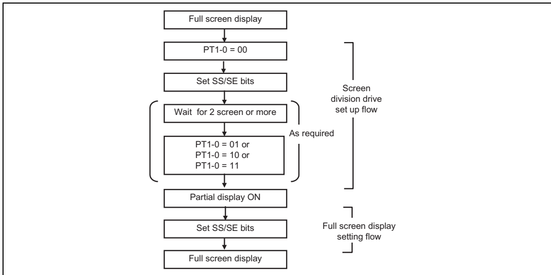
Partial display setting flow
