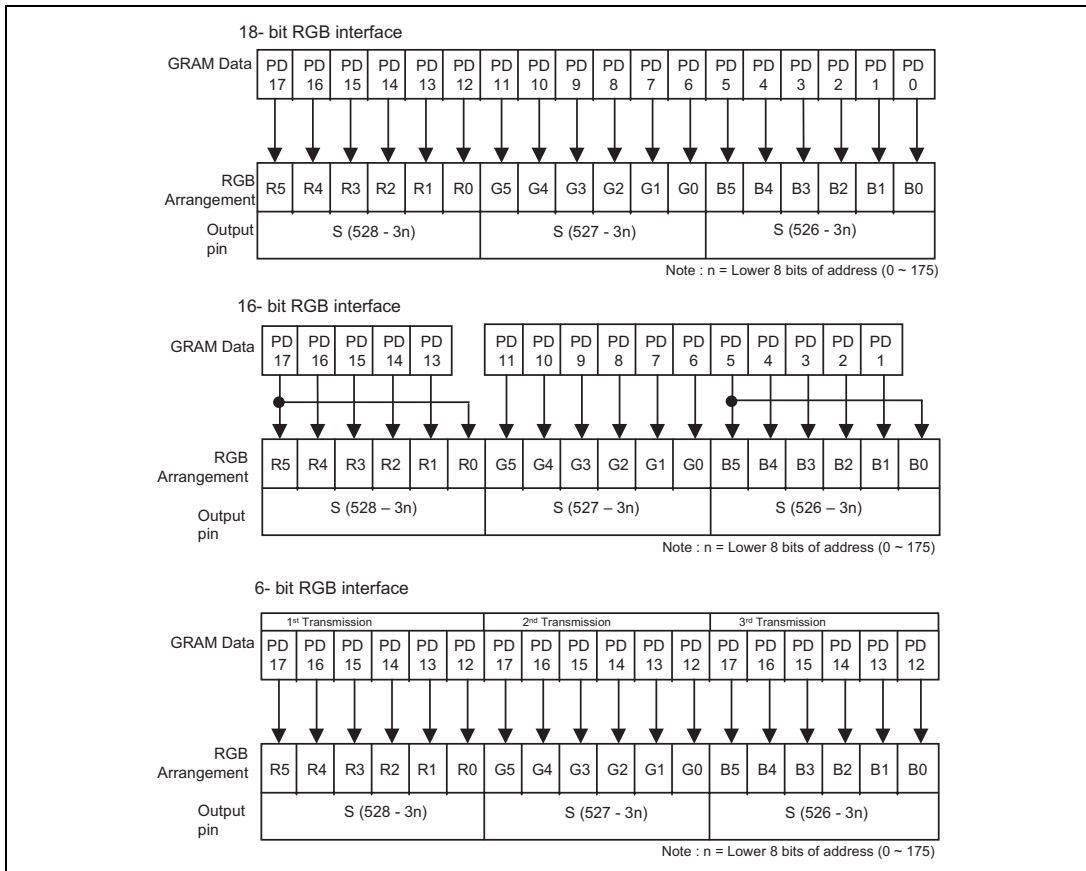
GRAM data and RGB assignment (SS = "1", BGR = "1")
