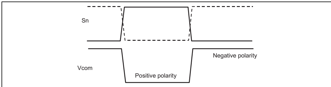
Source output and V_{com}
