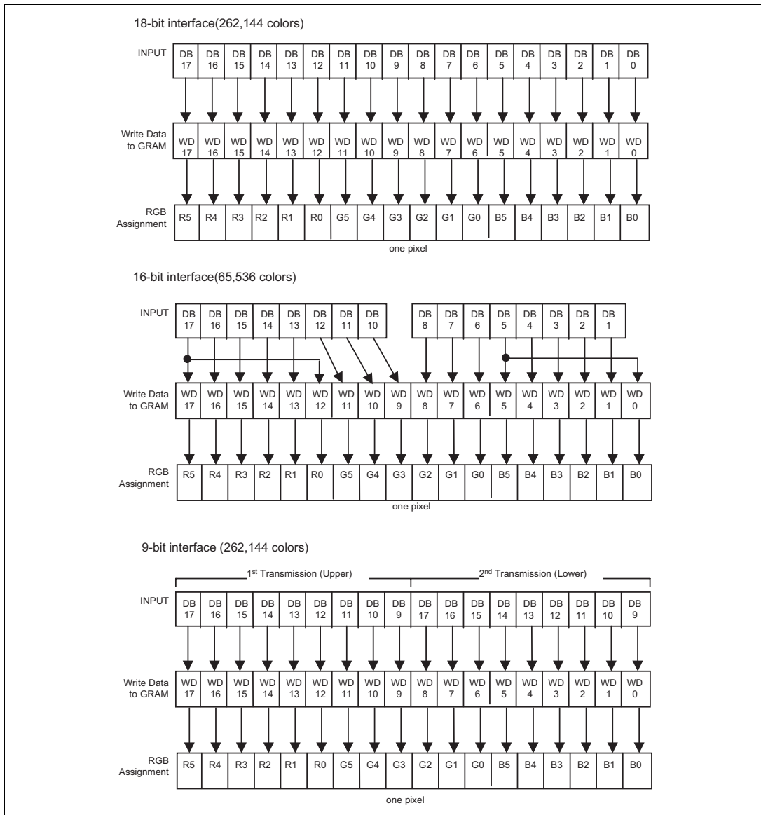
Write data to GRAM: Bit assignment
