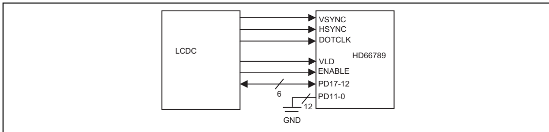
6-bit RGB interface
