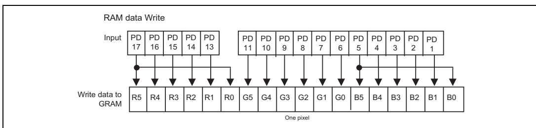
Data format for 16-bit interface
