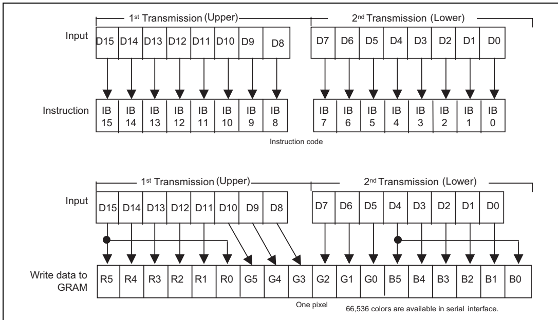
Data format for SPI
