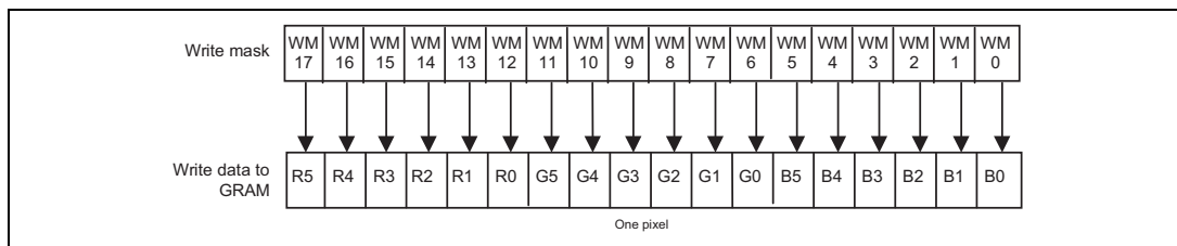
RAM write data mask
