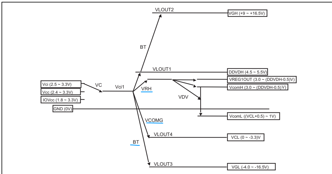
Pattern diagram for voltage setting
