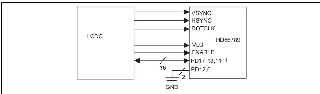
16-bit RGB interface
