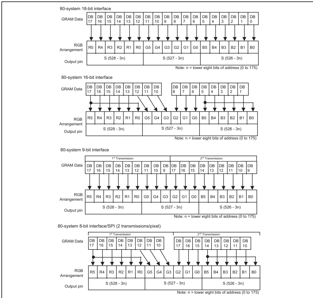
GRAM data and RGB assignment (SS = "1", BGR = "1")
