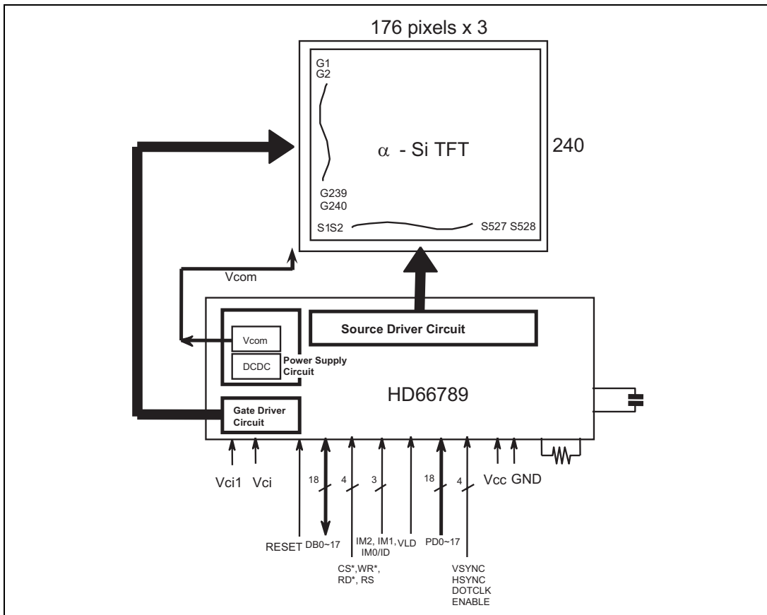
System configuration with HD66789
