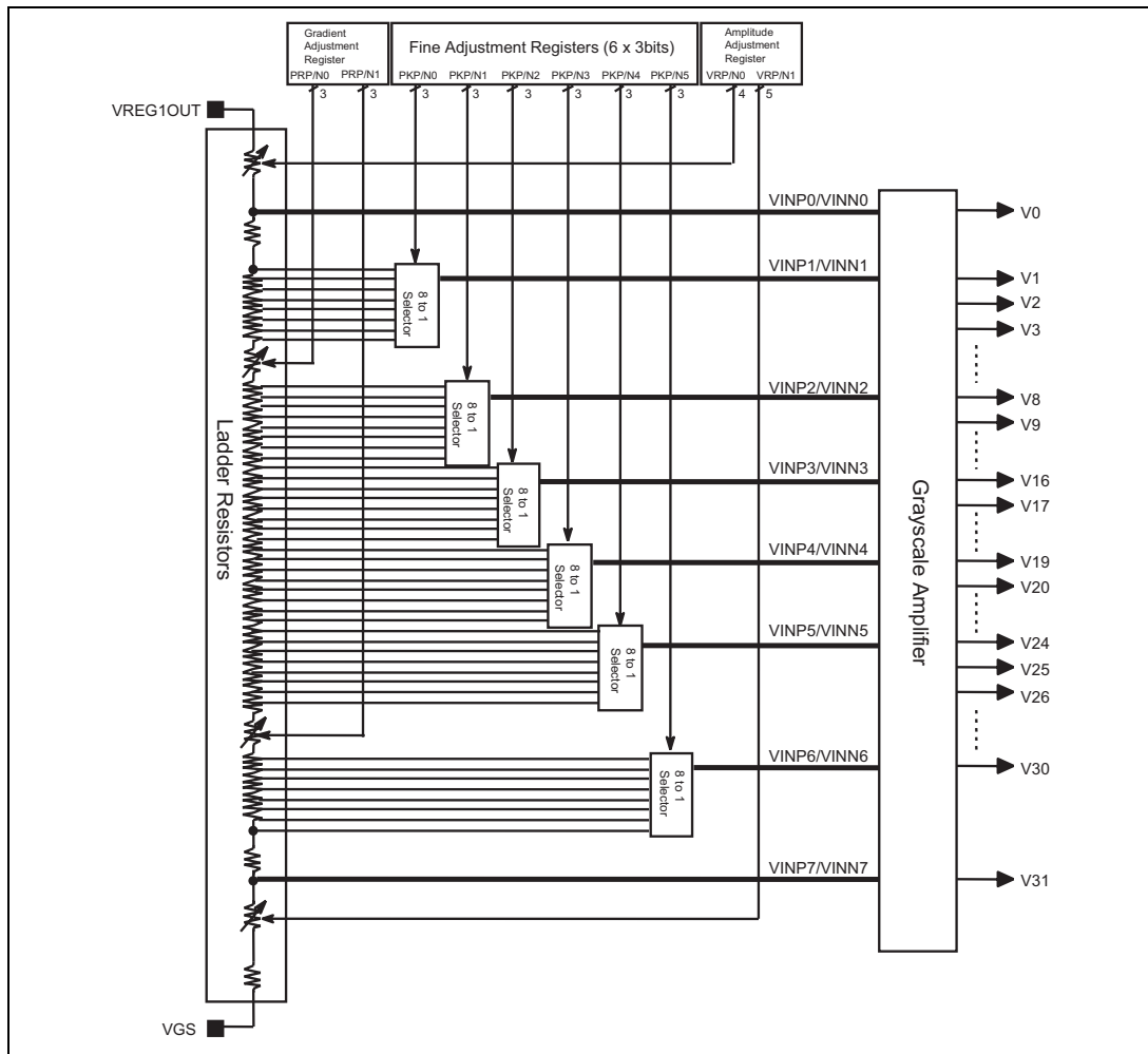
Grayscale amplifier
