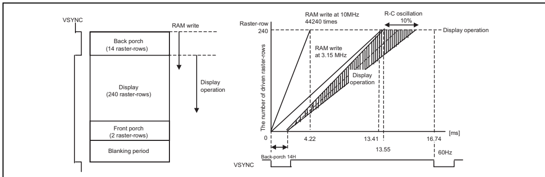
Operation through VSYNC interface
