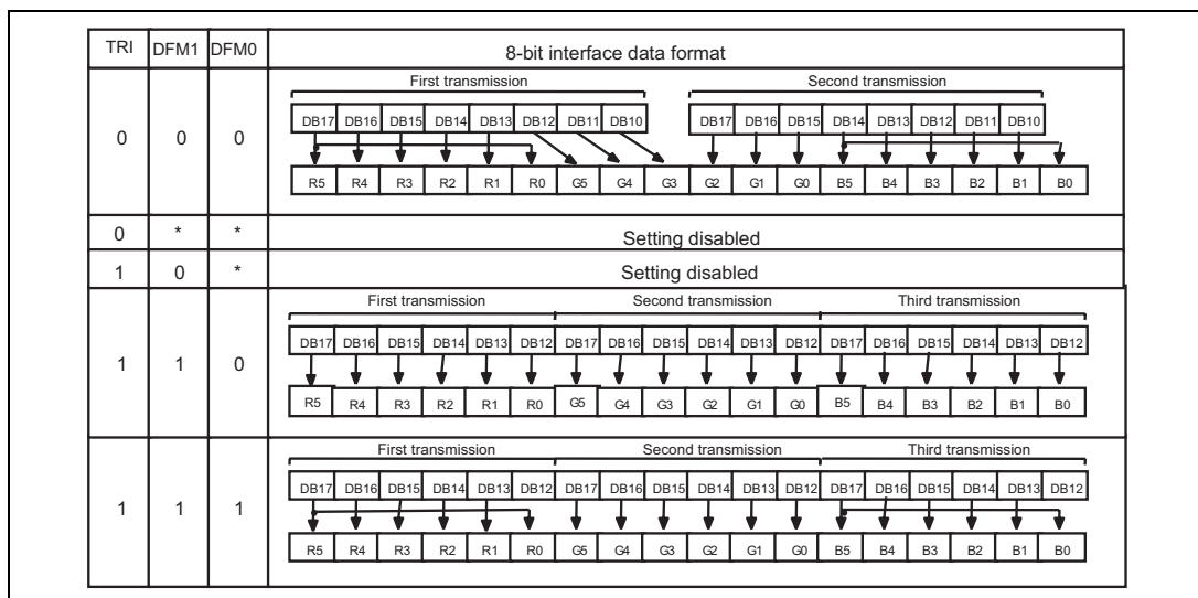
8-bit interface data format
