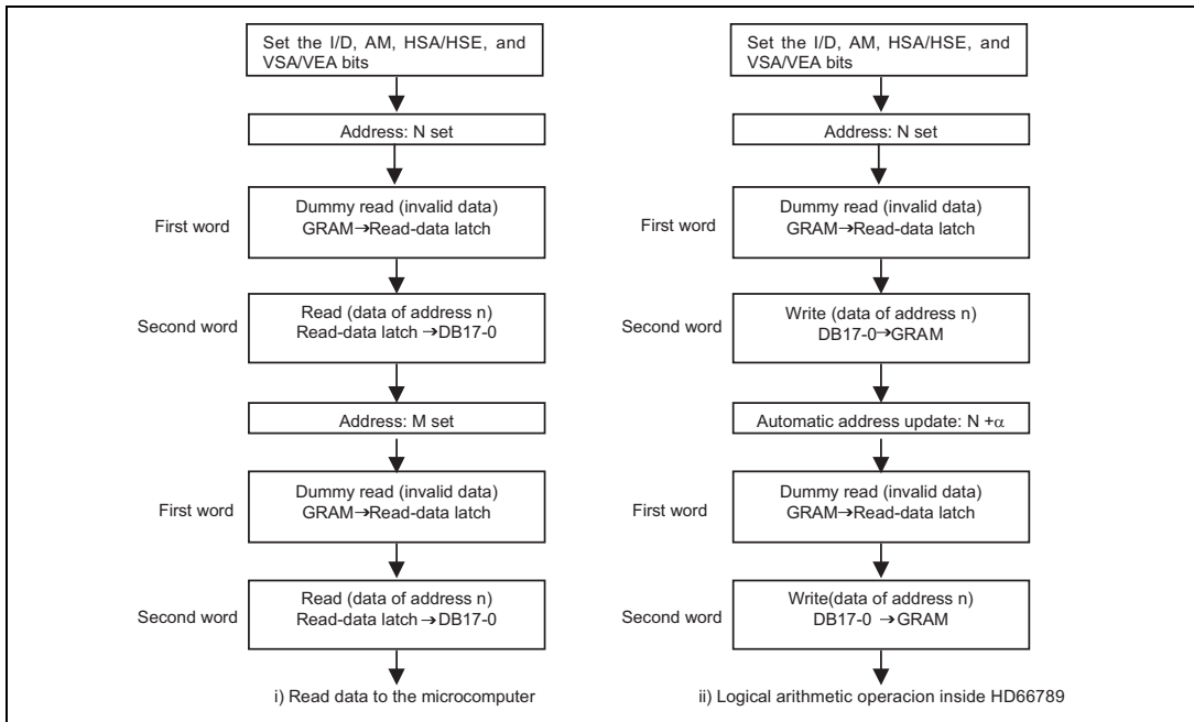
GRAM read sequence
