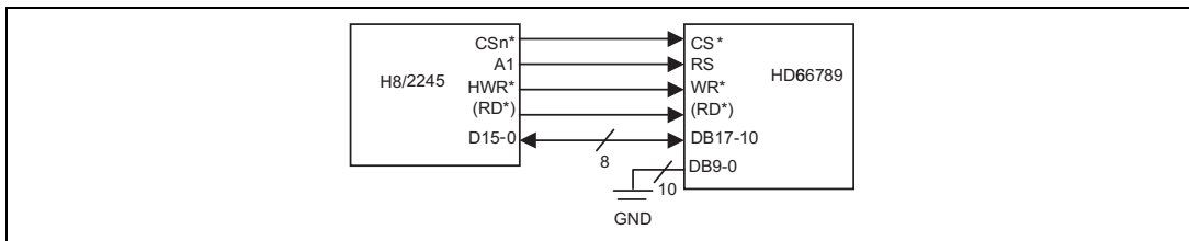
8-bit microcomputer and HD66789
