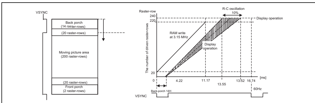
Limiting moving picture display area
