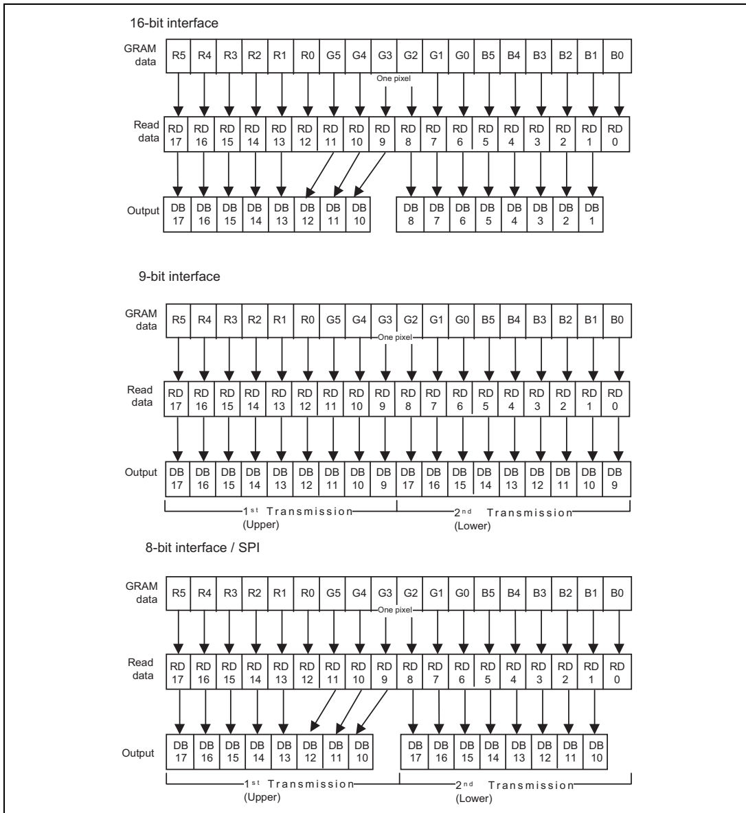
Read data from GRAM: Bit assignment
