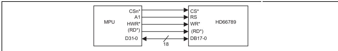
18-bit microcomputer and HD66789
