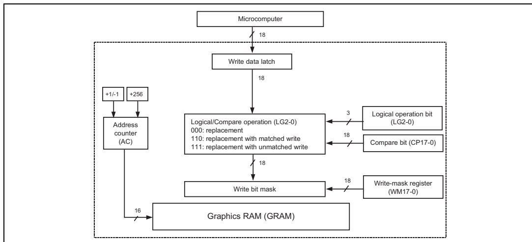
Graphics operation flow
