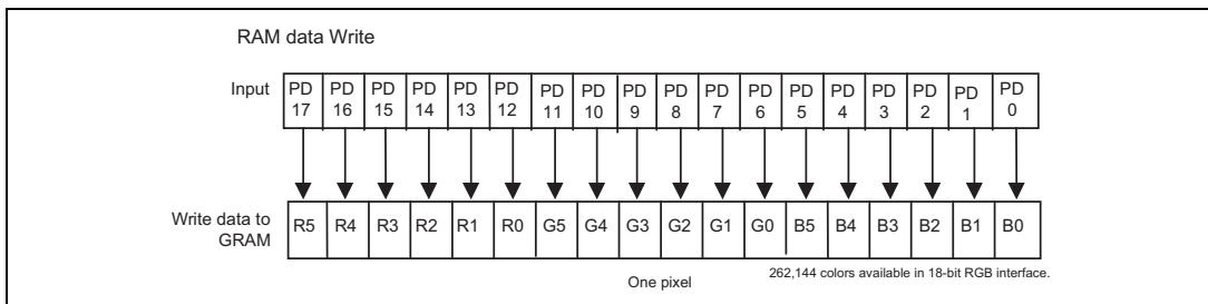
Data format for 18-bit interface
