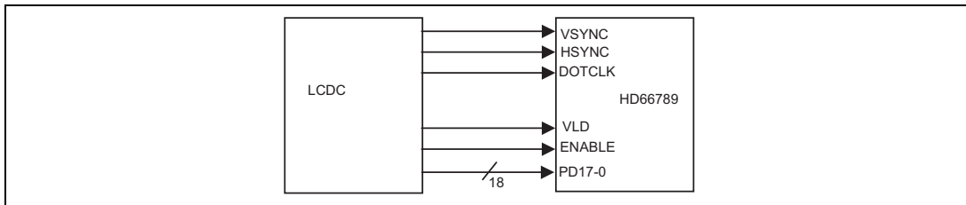
18-bit RGB interface
