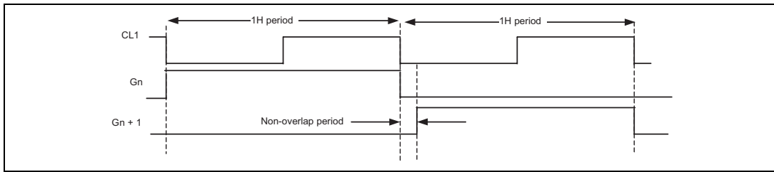
Non-overlap period
