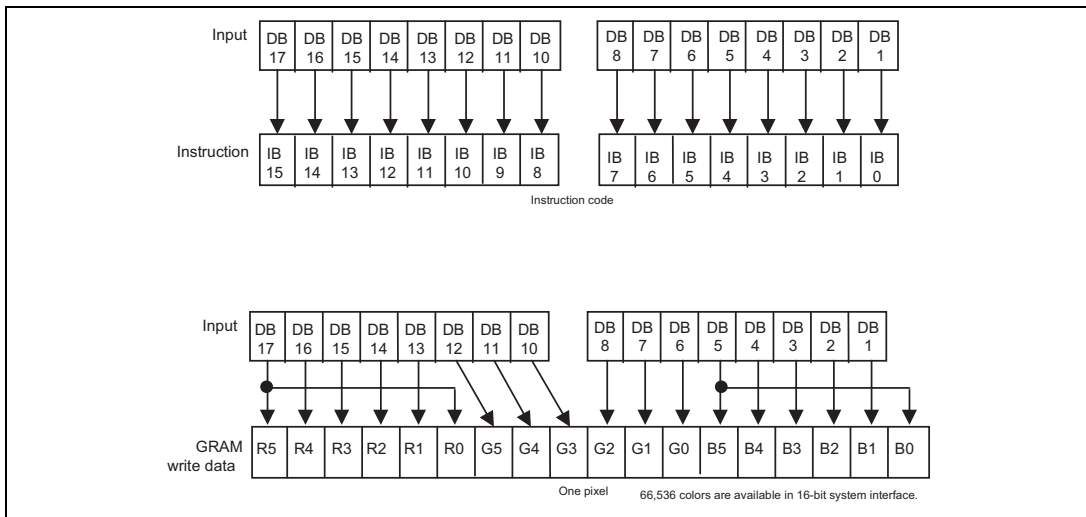
Data format for 16-bit interface
