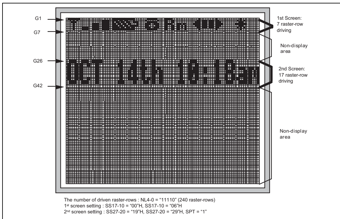
Screen-split Drive
