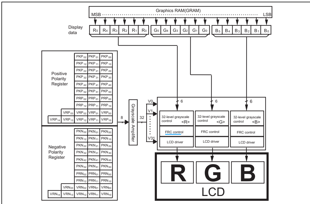
Grayscale control
