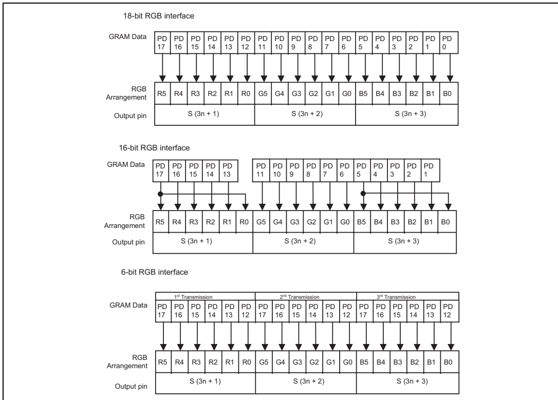
GRAM data and RGB assignment (SS = "0", BGR = "0")
