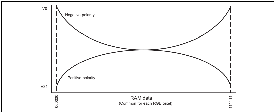
RAM data and the output voltage
