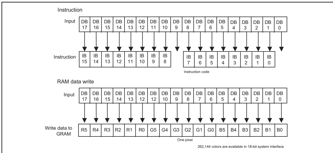
Data format for 18-bit interface
