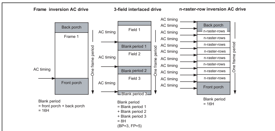
AC timing
