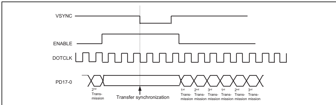
6-bit data transmission synchronization
