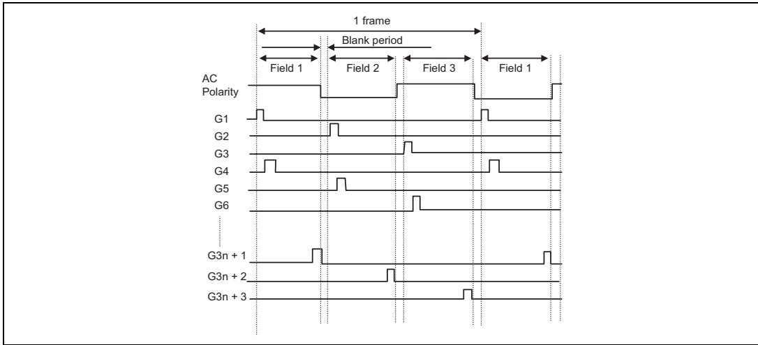
Gate output timing in 3-field interlaced drive
