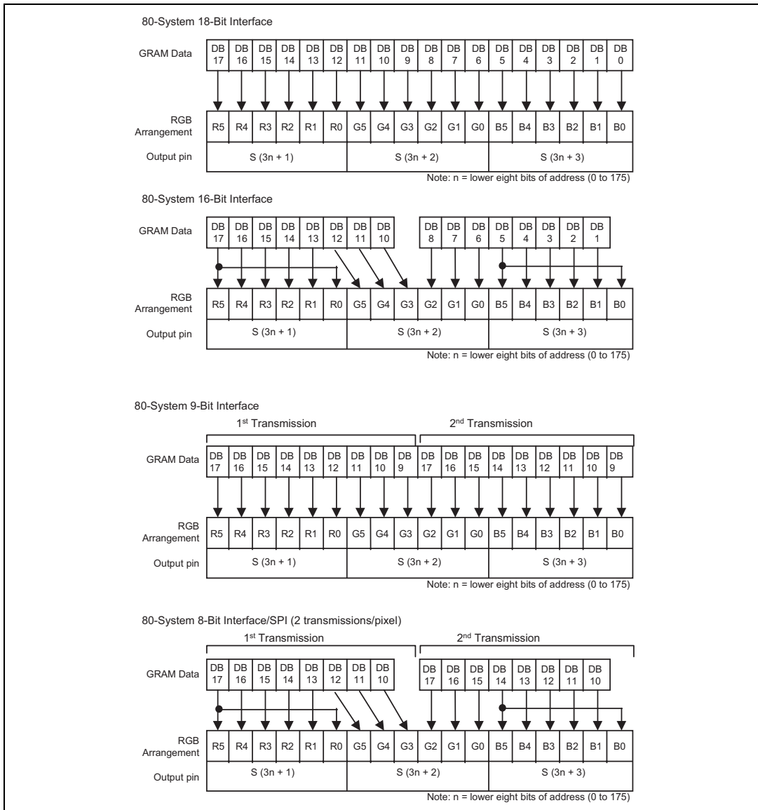
GRAM data and RGB assignment (SS = "0", BGR = "0")
