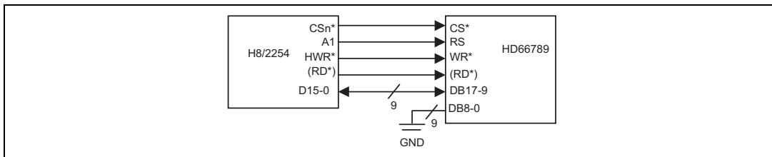
9-bit microcomputer and HD66789
