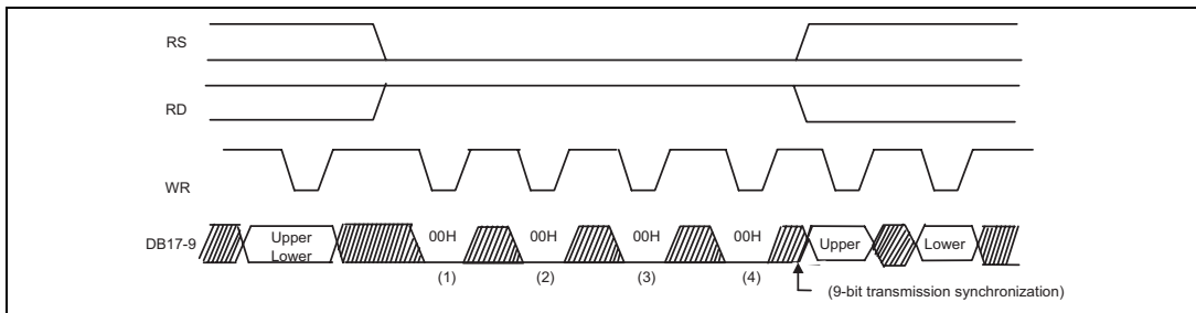
9-bit data transmission synchronization
