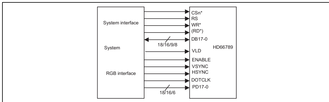
Interfaces and HD66789
