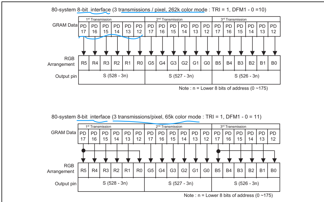
GRAM data and RGB assignment (SS = "1", BGR = "1")
