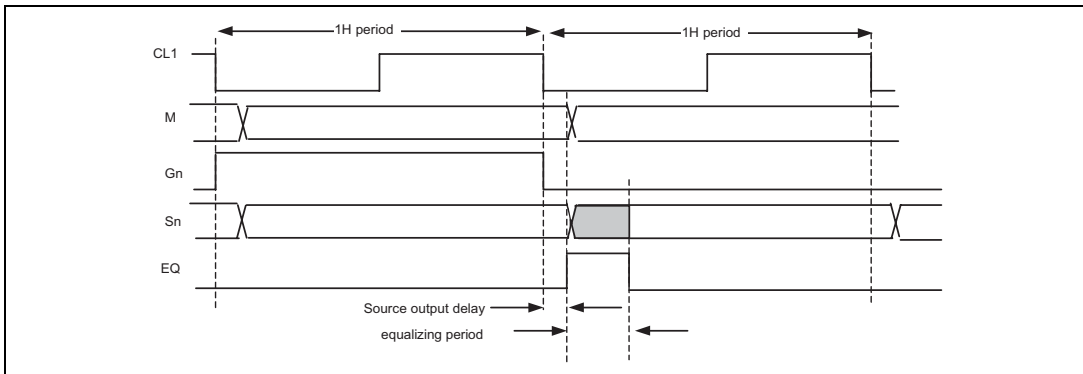
Source output delay and equalize period
