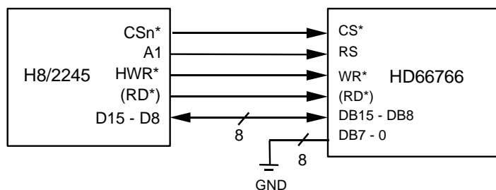
Figure 27 Interface to 8-bit Microcomputer
