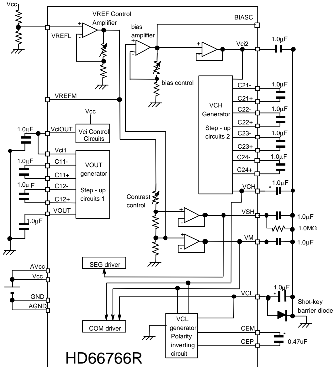
Figure 55 Configuration of internal power circuit
