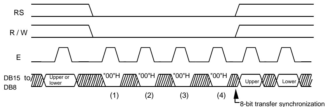
Figure 28 8-bit Transfer Synchronization
