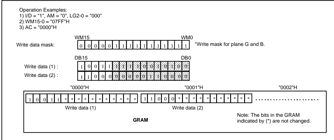
Figure 39 Writing Operation of Write Mode 1
