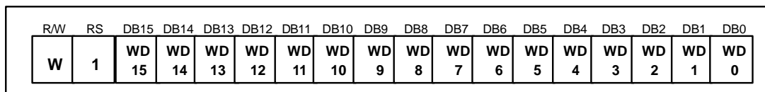
Figure 22 Write Data to GRAM Instruction
