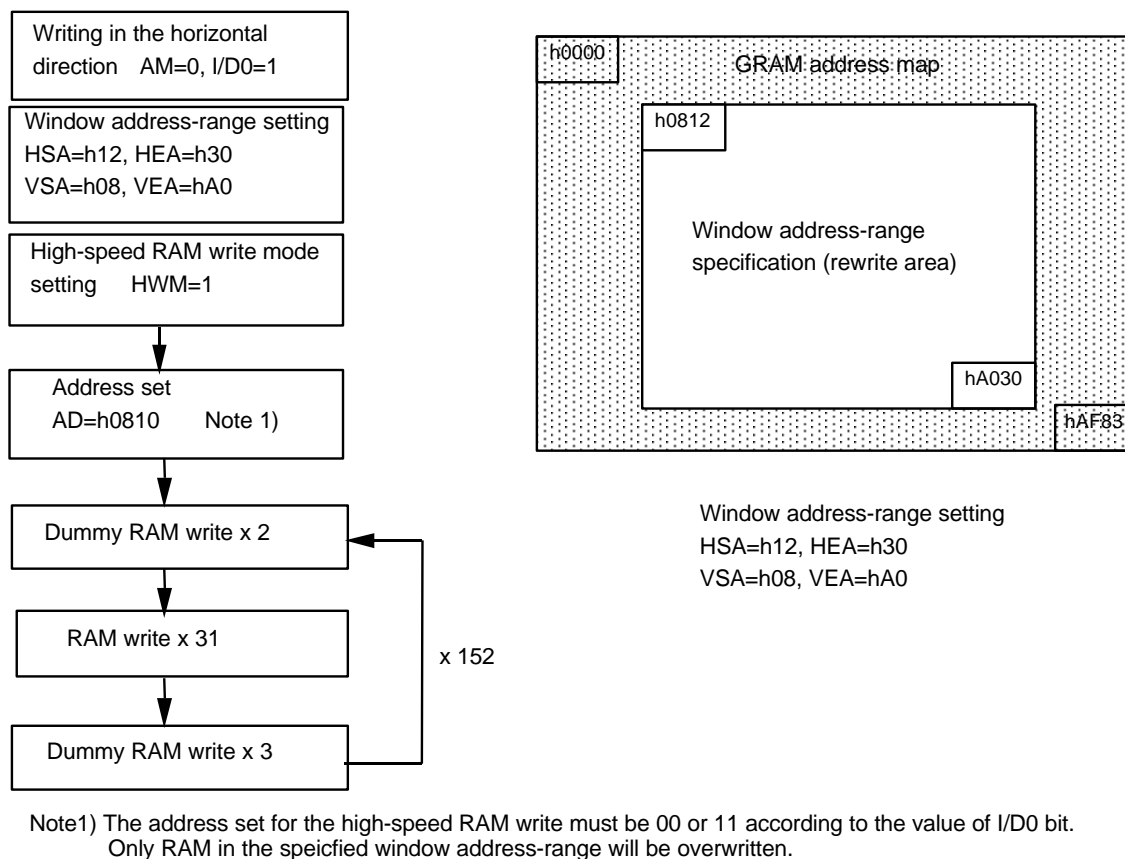
Figure 35 Example of the High-Speed RAM write with a window address-range specification
