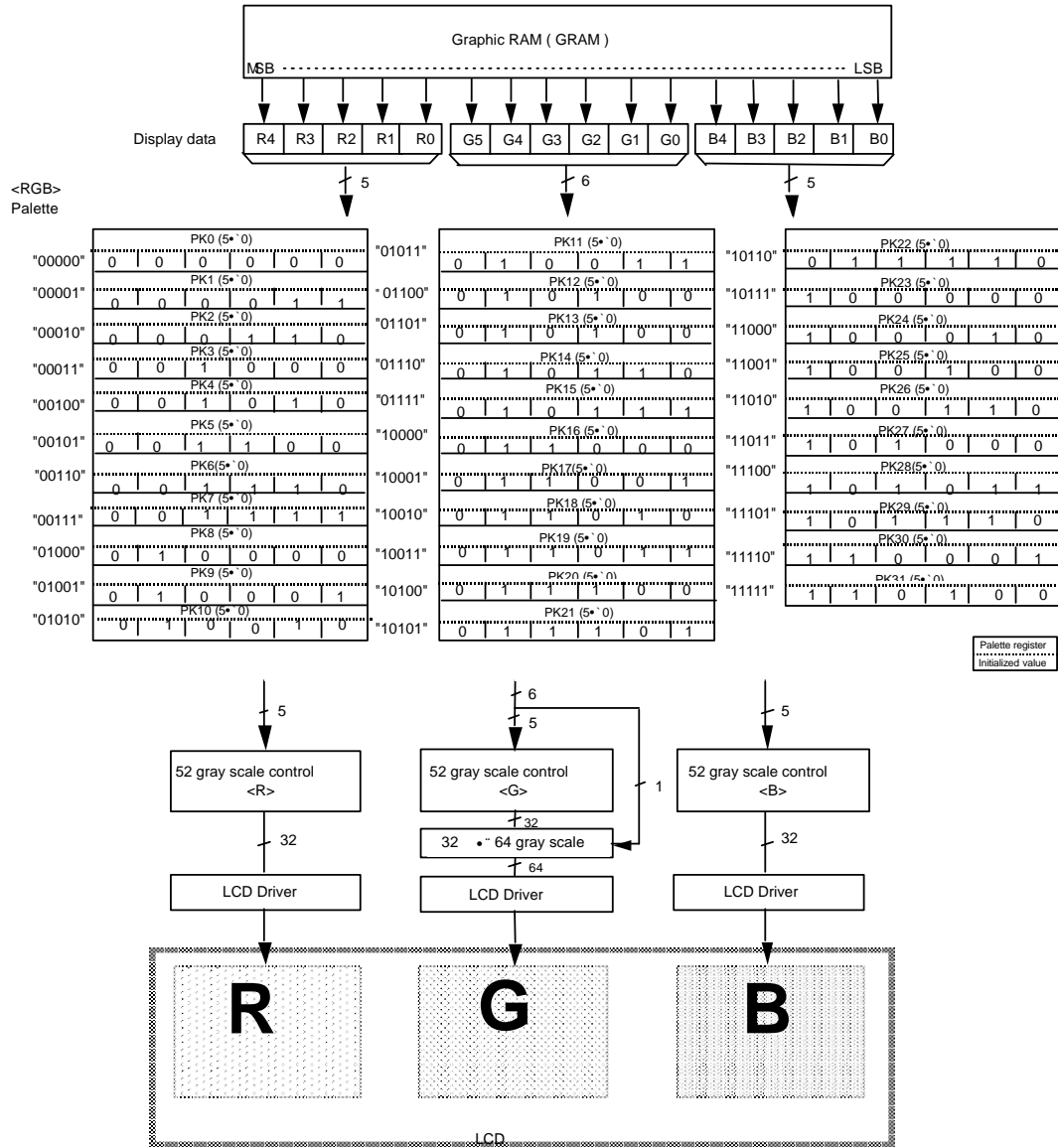
Figure 44 Grayscale Palette Control
