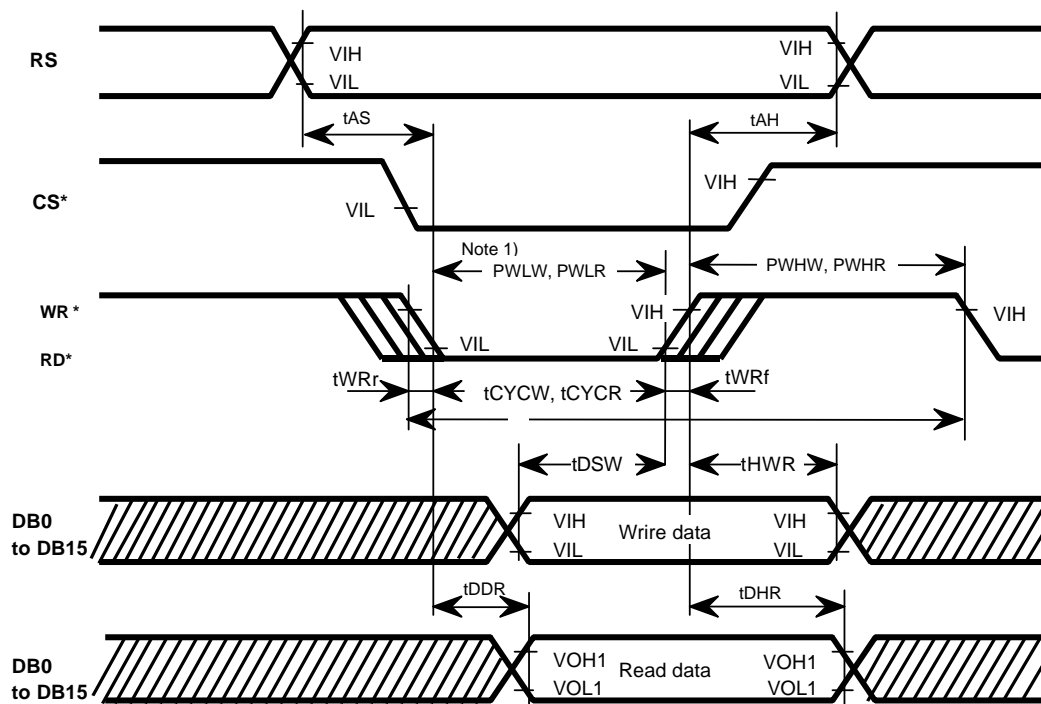
Figure 80 80-system Bus Timing
