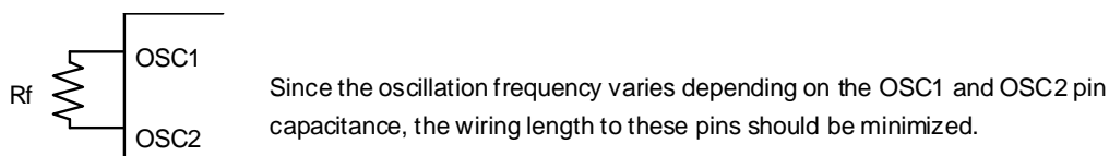
Figure 68 Internal Oscillation
