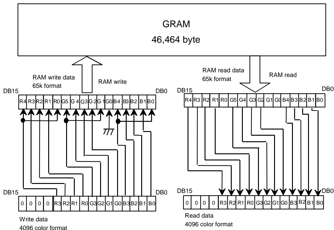
Figure 43 4096 color display data write and read format
