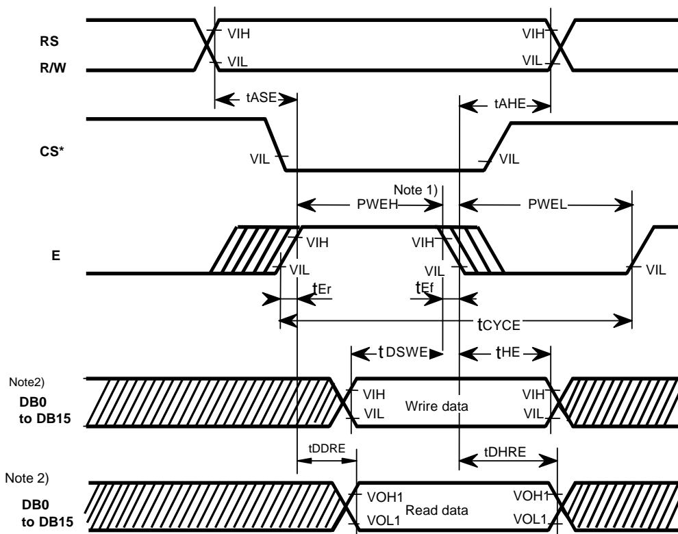
Figure79 68-system Bus Timing
