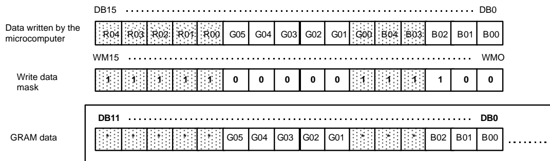
Figure 38 Write-data Mask Function Operation
