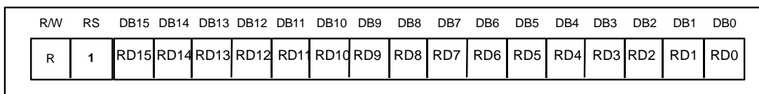
Figure 24 Read Data from GRAM Instruction
