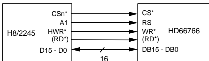
Figure 26 Interface to 16-bit Microcomputer
