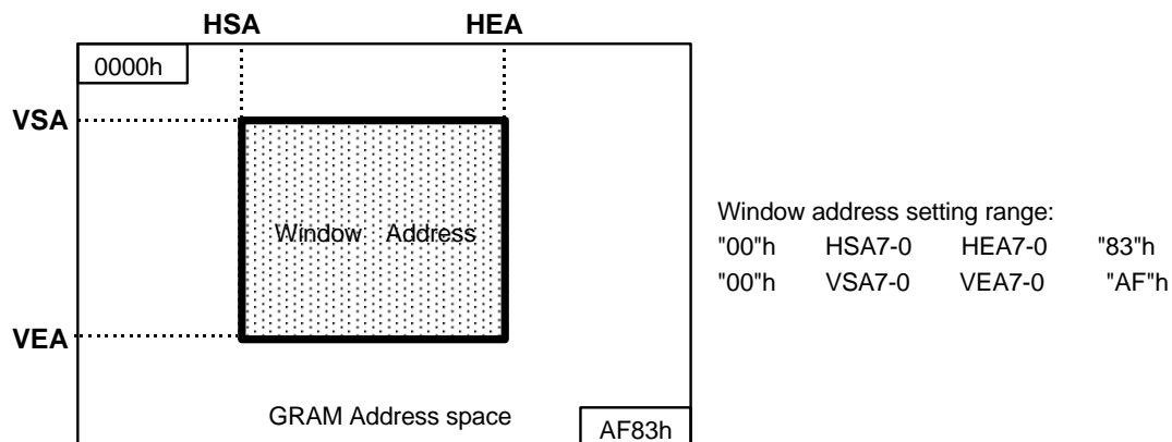
Figure 19 Window Address Setting Range
