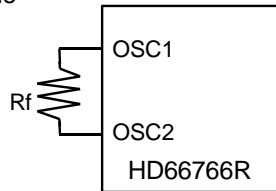
Figure 51 Oscillation Circuits
