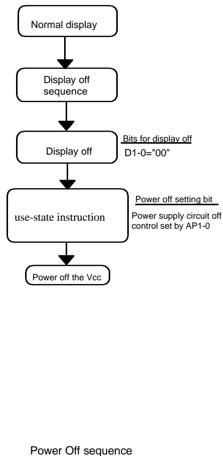
Figure 47 Power-off Sequence
