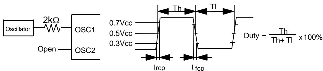
Figure 67 External Clock Supply
