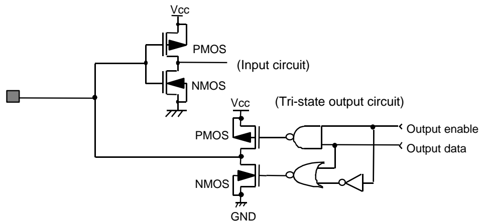
Figure 66 I/O Pin Configuration
