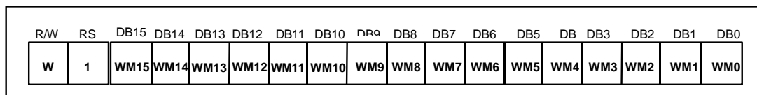
Figure 20 RAM Write Data Mask Instruction
