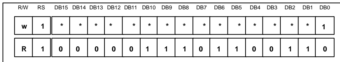
Figure 6 Start Oscillation Instruction
