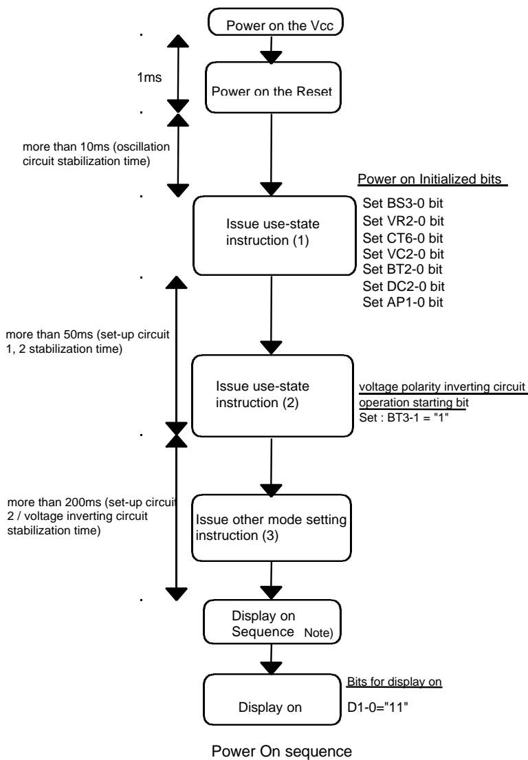
Figure 46 Power-on Sequence
