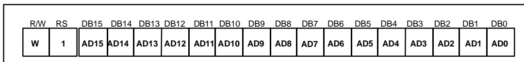
Figure 21 RAM Address Set Instruction
