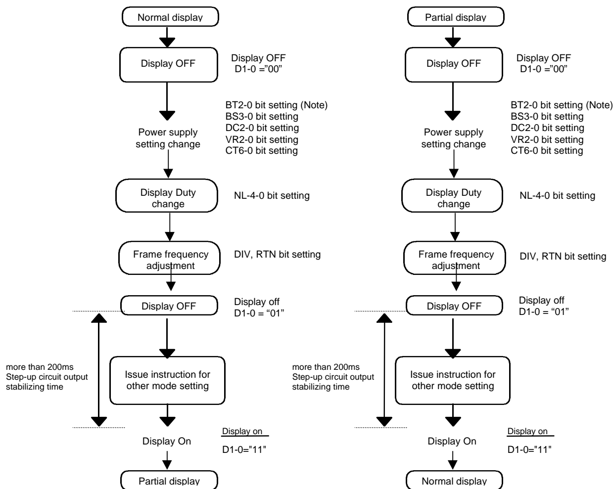
Figure 49 Normal to partial display
