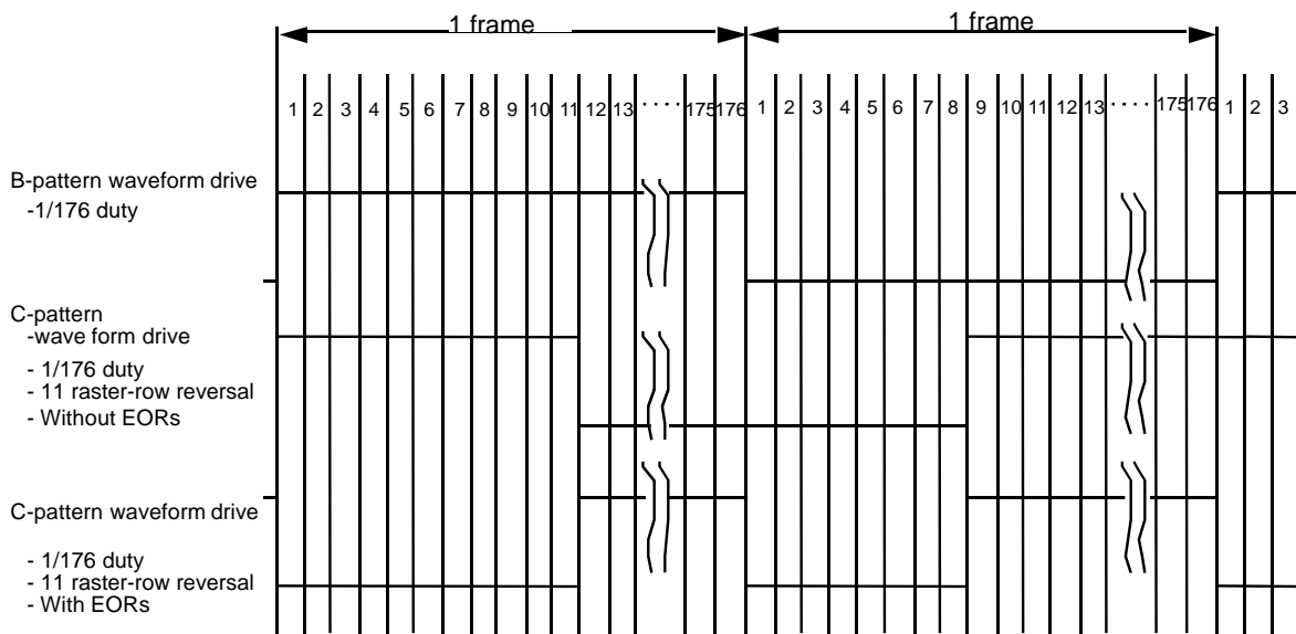
Figure 53 Example of an AC Signal under n-raster-row Reversed AC Drive
