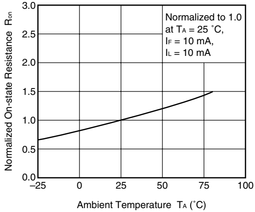
NORMALIZED ON-STATE RESISTANCE vs. AMBIENT TEMPERATURE
