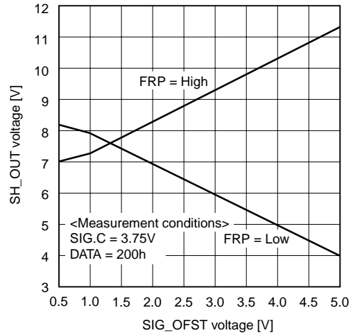
SIG_OFST voltage vs. SH_OUT voltage
