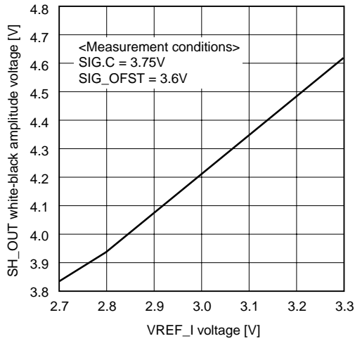
VREF_I voltage vs. SH_OUT voltage white-black amplitude
