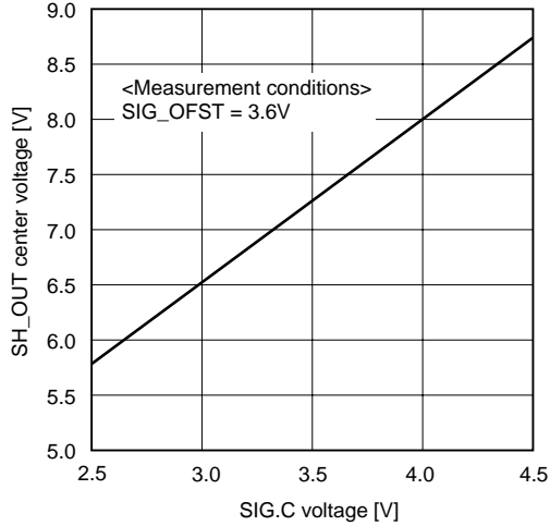
SIG.C voltage vs. SH_OUT center voltage
