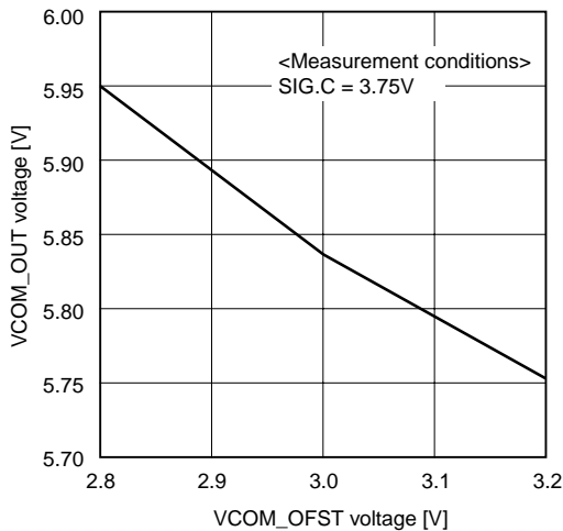
VCOM_OFST voltage vs. VCOM_OUT voltage
