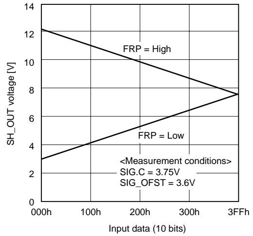
Input data vs. SH_OUT voltage
