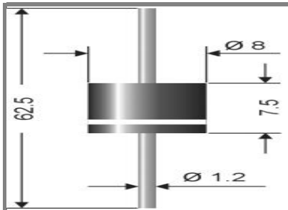
Axial lead diode
