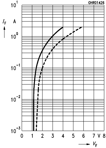
Forward current
