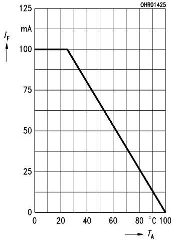
Max. forward current
