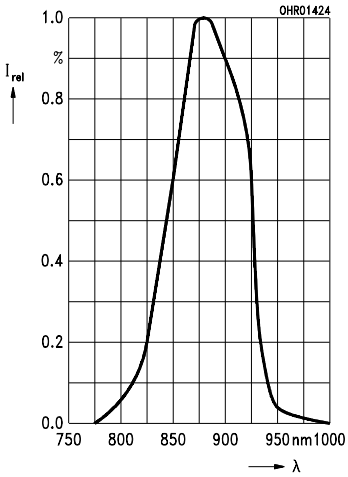
Relative spectral emission
