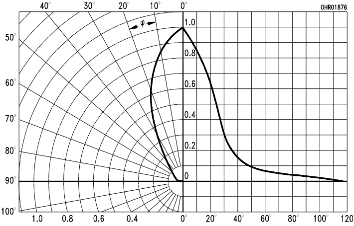
Directional characteristics I_{rel} = f(\varphi)
