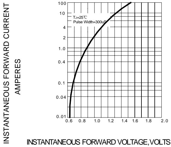
FIG.1 – FORWARD CHARACTERISTIC
