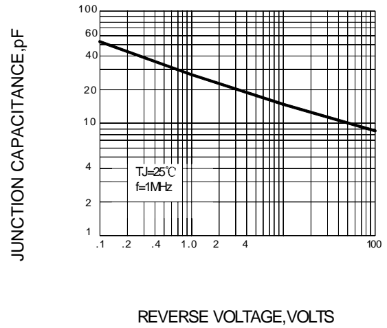
FIG.2 – JUNCTION CHARACTERISTICS
