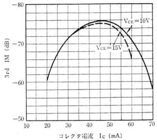
3rd ORDER IM DISTORTION vs. COLLECTOR CURRENT
