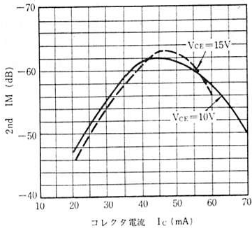
2nd ORDER IM DISTORTION vs. COLLECTOR CURRENT
