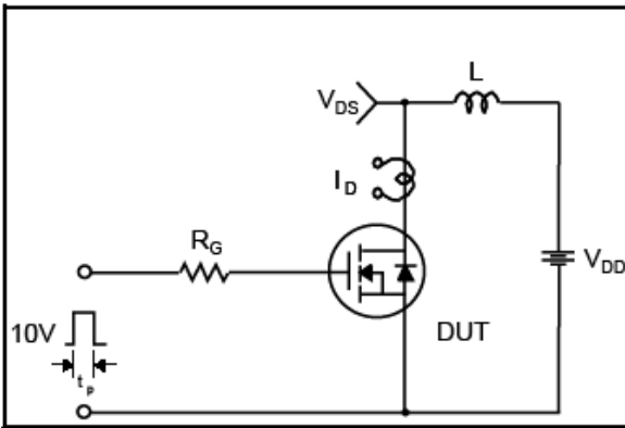
Fig 15. Unclamped Inductive Switching Test Circuit
