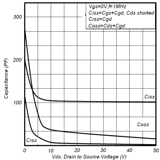
Fig 8. Capacitance Characteristics
