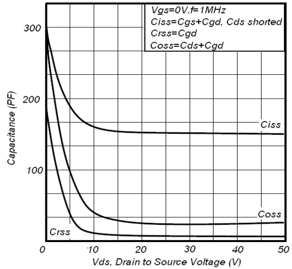
Fig 8. Capacitance Characteristics
