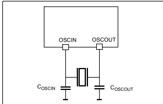
Figure 11. Crystal/Ceramic Resonator
