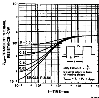
Figure 12 Transient Thermal Resistance vs Time for MTP3N35/3N40
