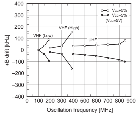
Oscillation frequency power supply fluctuation (PLL off)
