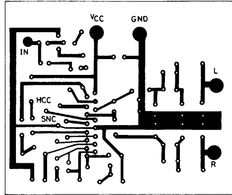
Sample printed circuit pattern
