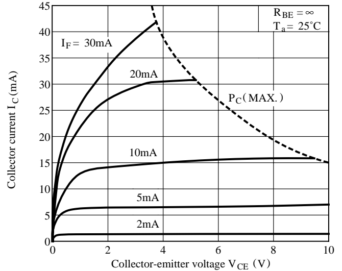
Fig. 6 Collector Current vs. Collector-emitter Voltage
