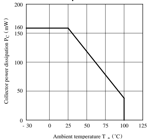
Fig.12 Collector Power Dissipation VS. Ambient Temperature
