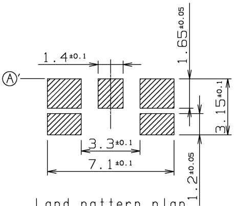
Land pattern plan
