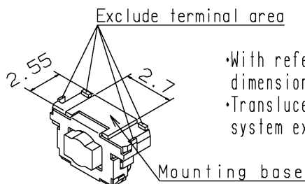
Fig.4 Recognition position of Switch
