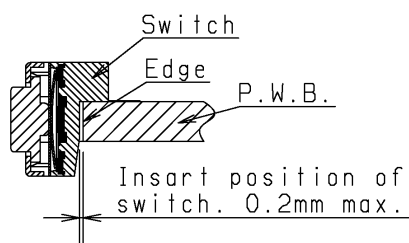
Fig.5. Mounting(Insert) Position
