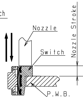
Fig.6 Nozzle stroke
