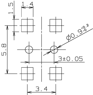
P.C.B.piercing plan (Tolerance : \pm 0.1 )
