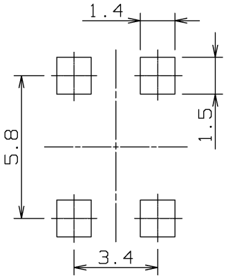
P.C.B.piercing plan (Tolerance : \pm 0.1 )
