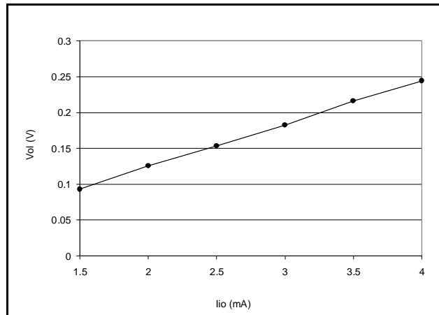
Figure 64. Typical V_{OL} at V_{DD}=5V (standard)
