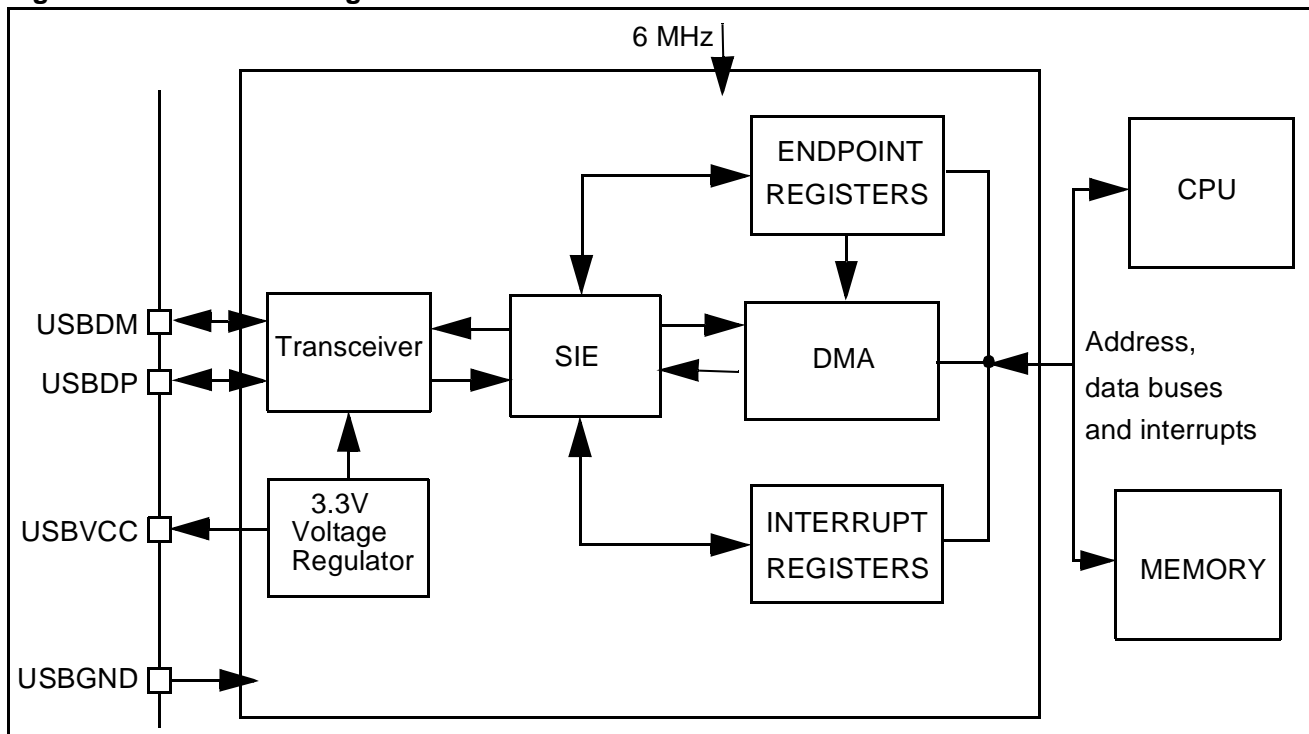
Figure 37. USB Block Diagram
