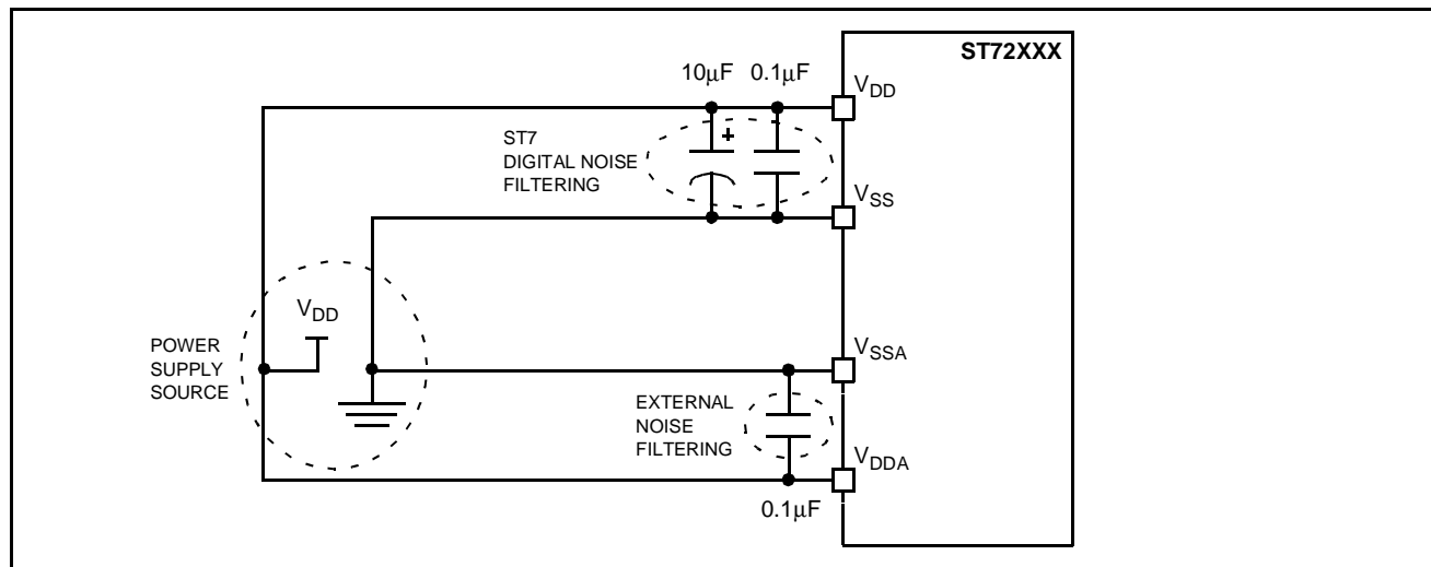
Figure 53. EMC Recommended star network power supply connection 2)
