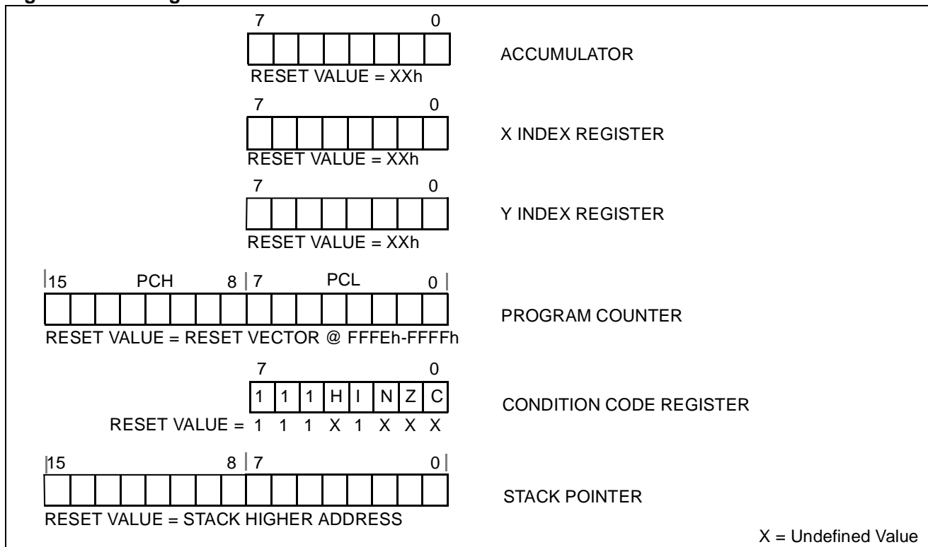
Figure 7. CPU Registers
