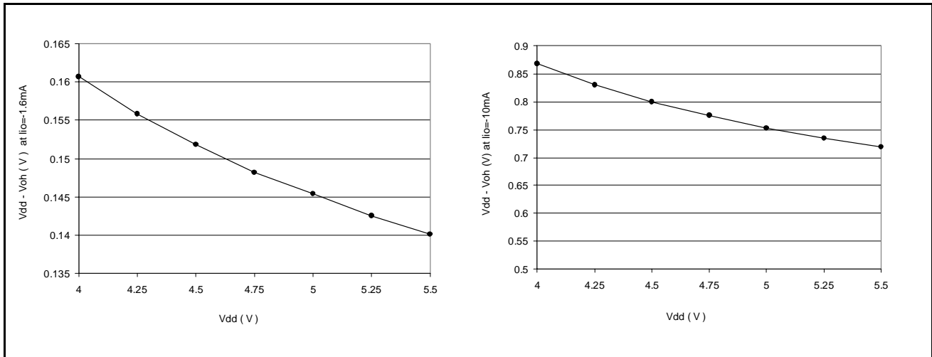
Figure 71. Typical V_{DD}-V_{OH} vs. V_{DD}
