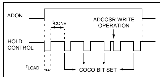
Figure 44. ADC Conversion Timings
