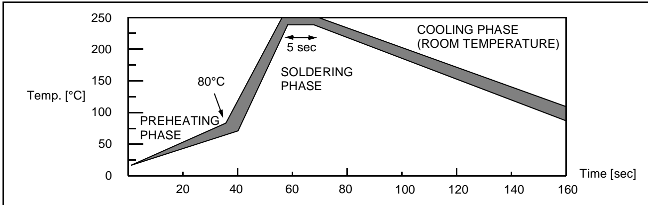
Figure 83. Recommended Reflow Soldering Oven Profile (MID JEDEC)
