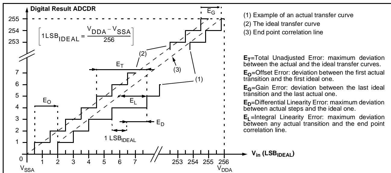
Figure 79. ADC Accuracy Characteristics
