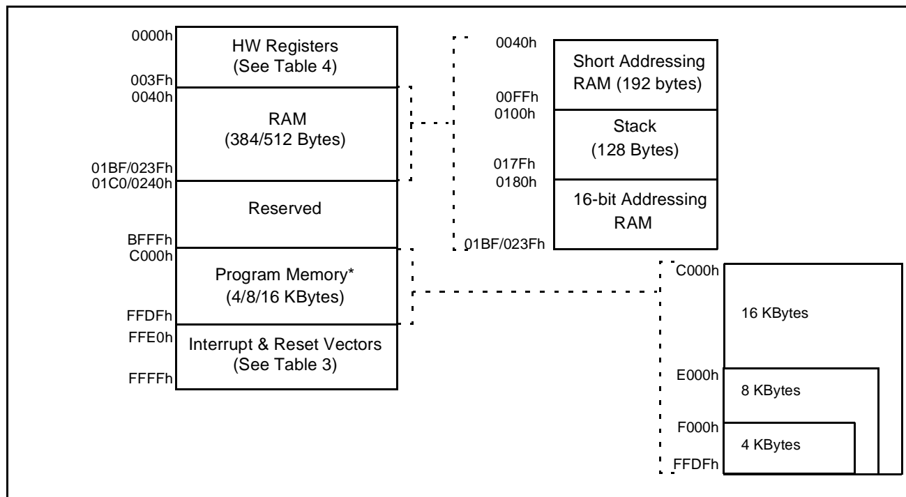
Figure 4. Memory Map
