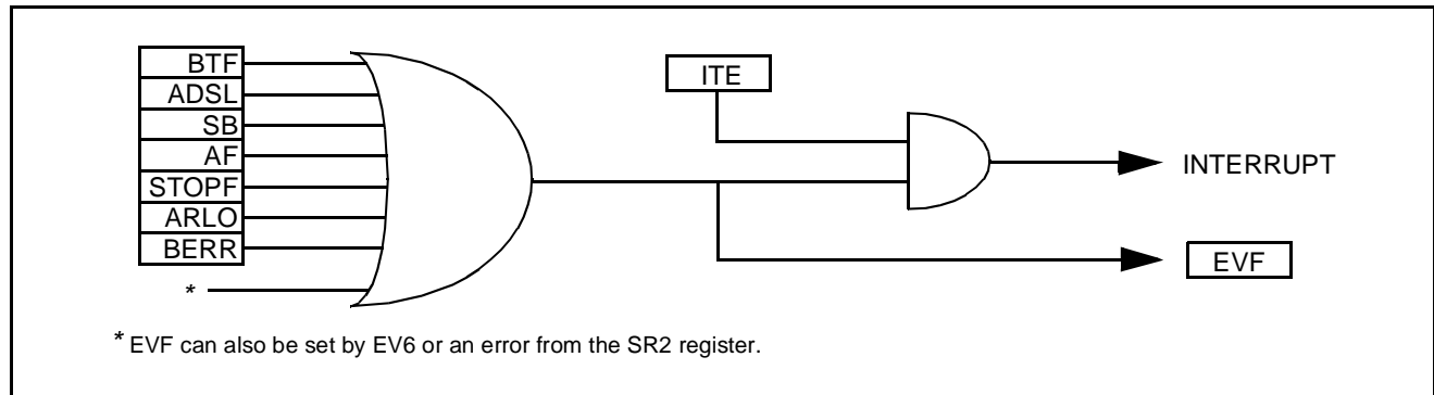
Figure 42. Event Flags and Interrupt Generation
