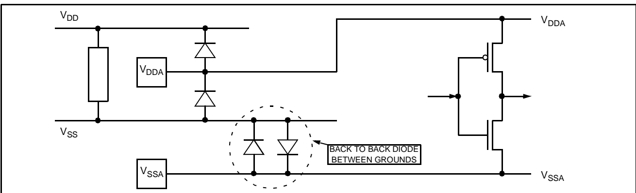
Figure 60. Multisupply Configuration
