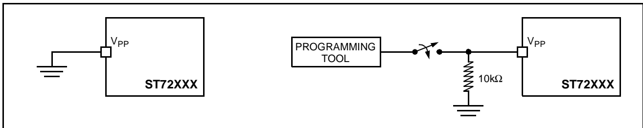
Figure 52. Two typical Applications with V_{PP} Pin 1)
