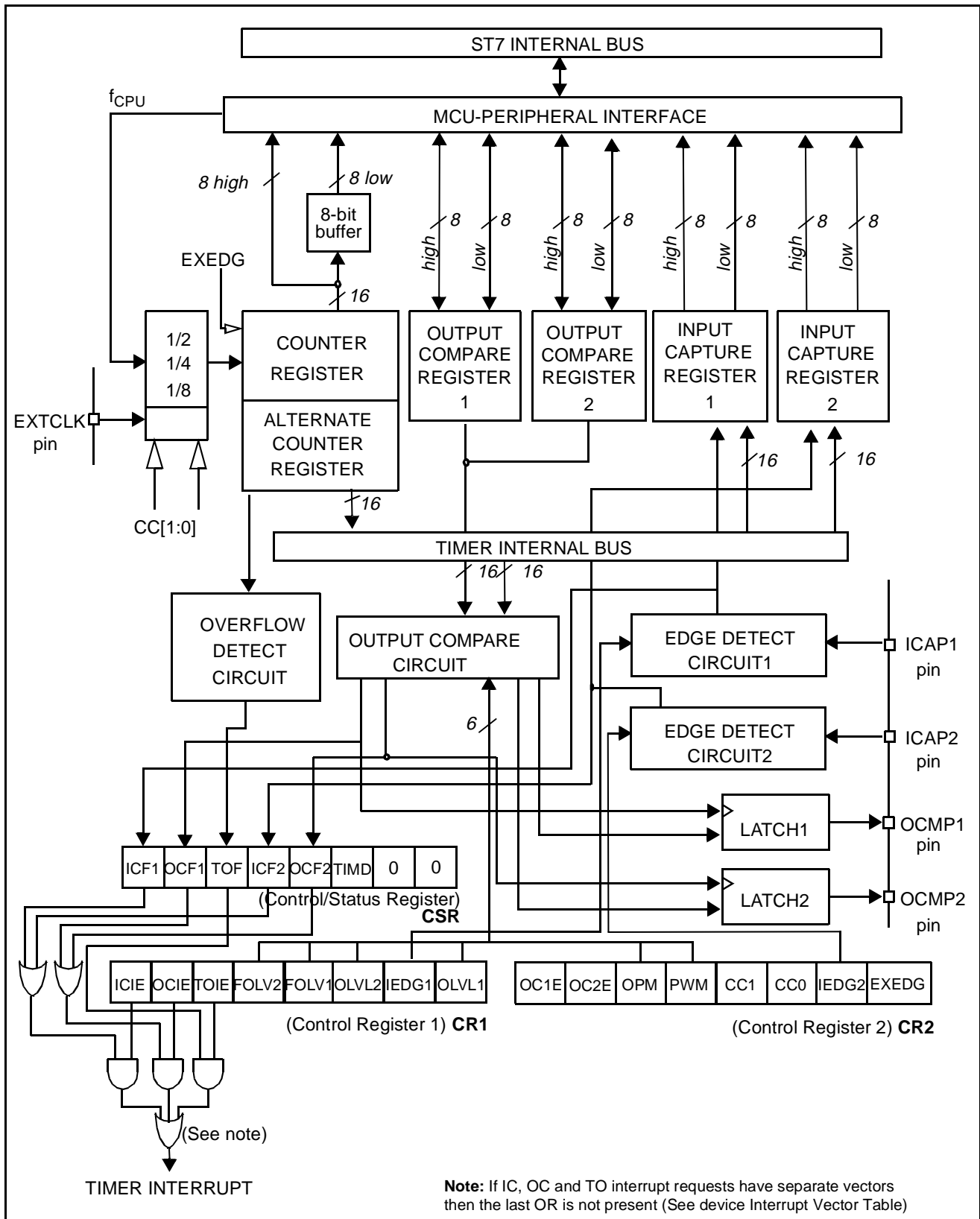
Figure 24. Timer Block Diagram
