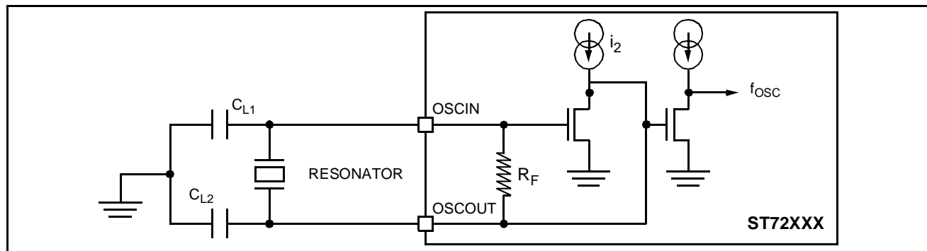
Figure 51. Typical Application with a Crystal Resonator
