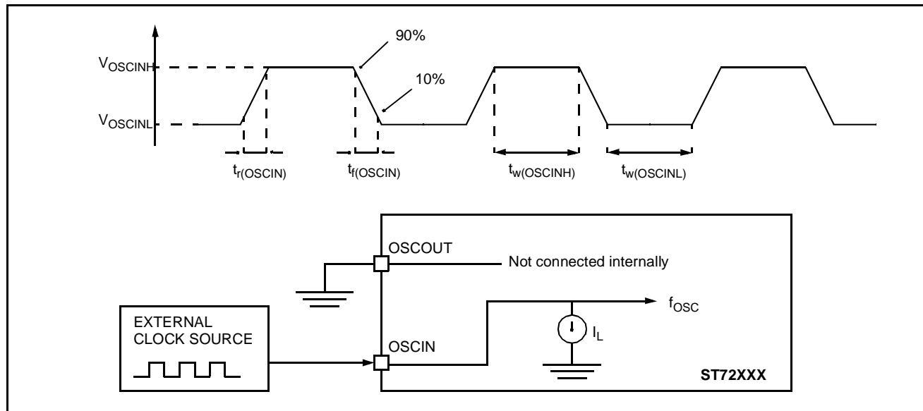
Figure 50. Typical Application with an External Clock Source
