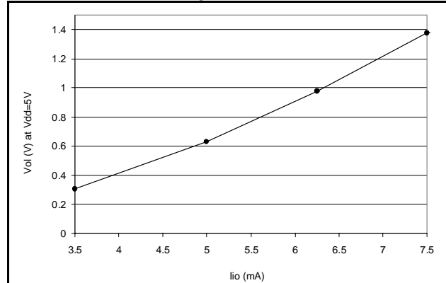
Figure 74. Typical V_{OL} at V_{DD}=5V ( \overline{RESET} )
