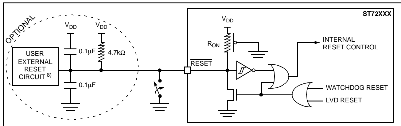
Figure 72. Typical Application with \overline{\text{RESET}} pin 7)
