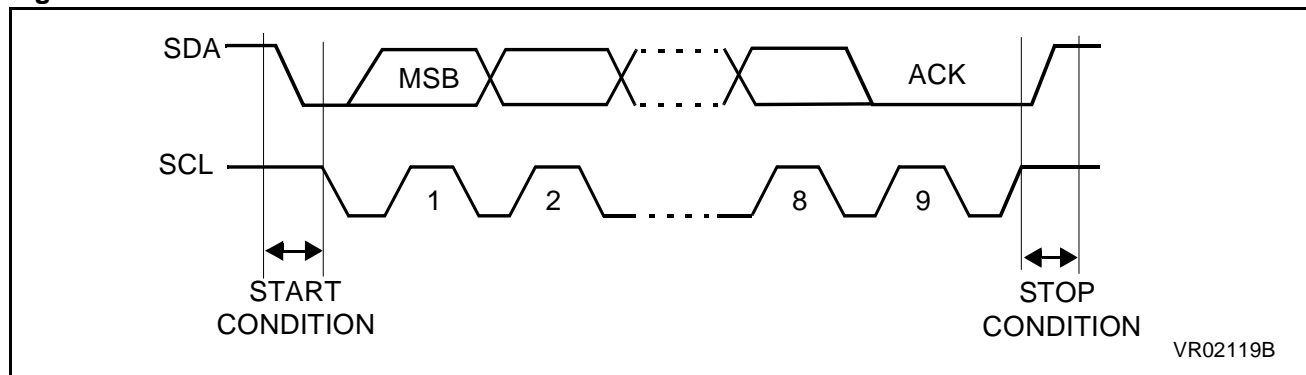
Figure 39. I 2 C BUS Protocol
