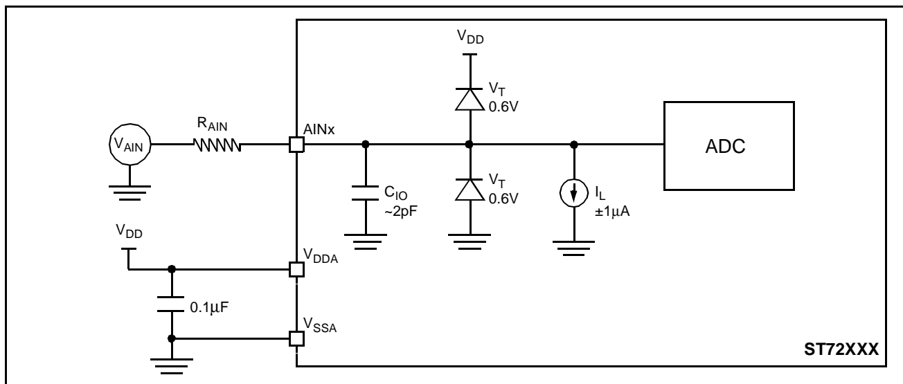
Figure 78. Typical Application with ADC
