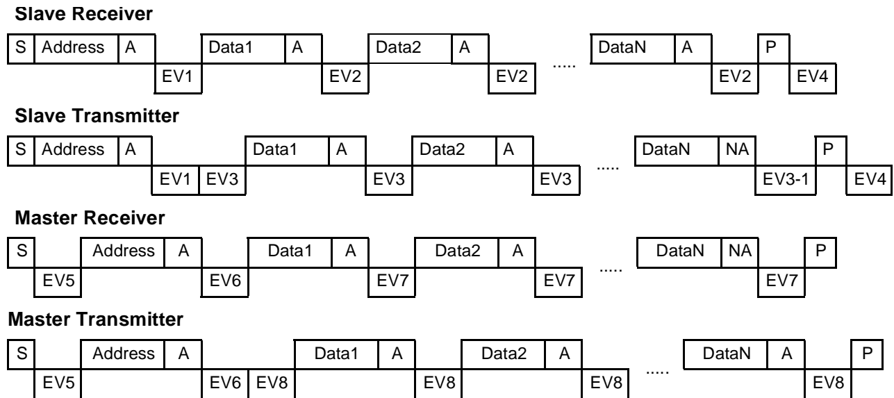
Figure 41. Transfer Sequencing
