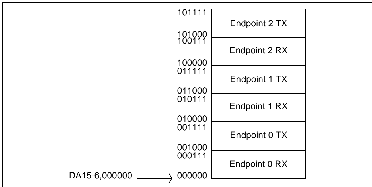
Figure 38. DMA Buffers
