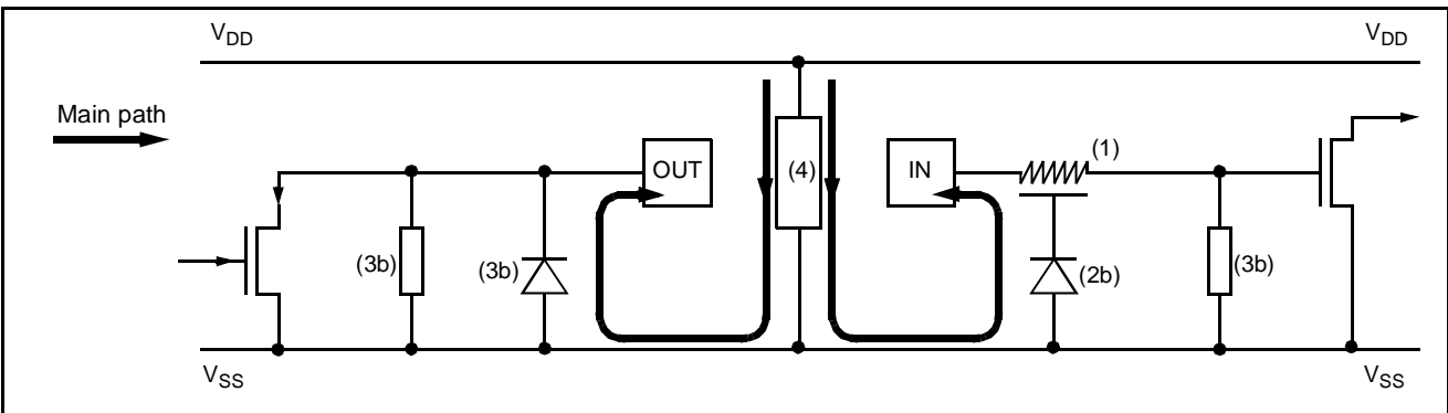
Figure 60. Multisupply Configuration
