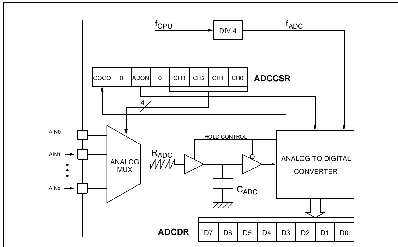
Figure 43. ADC Block Diagram
