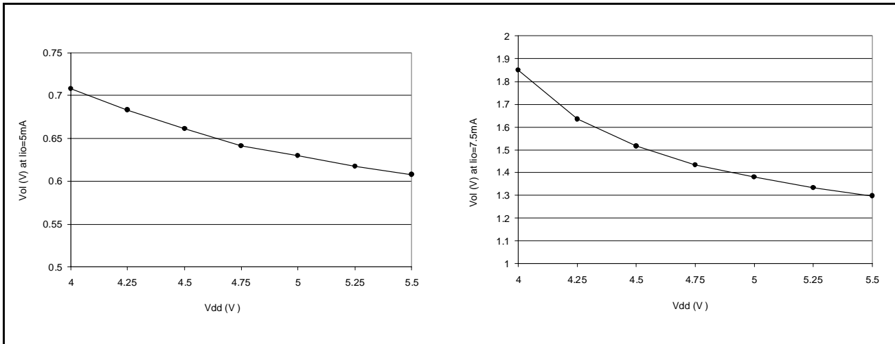
Figure 75. Typical V_{OL} vs. V_{DD} ( \overline{RESET} )
