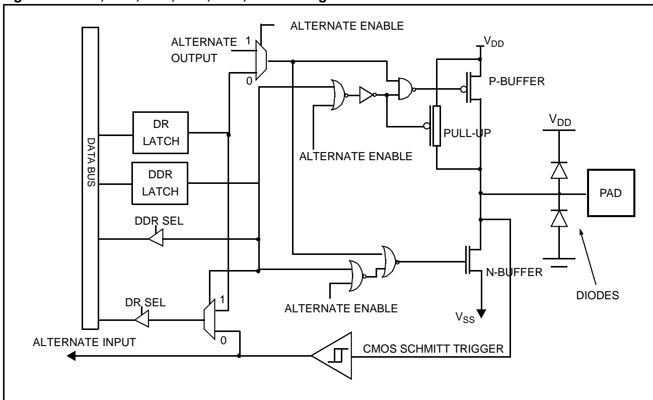
Figure 19. PA0, PA3, PA4, PA5, PA6, PA7 Configuration
