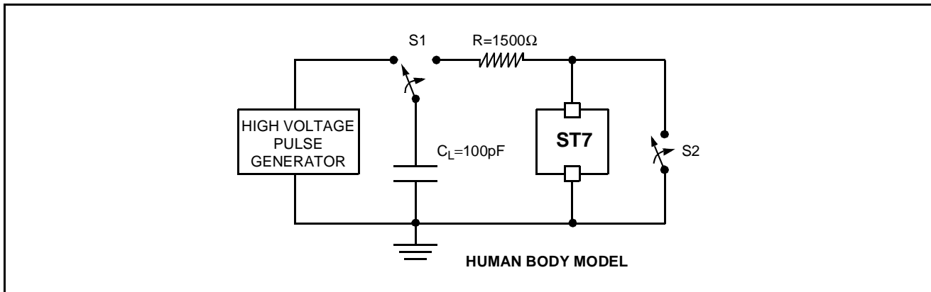
Figure 54. Typical Equivalent ESD Circuits
