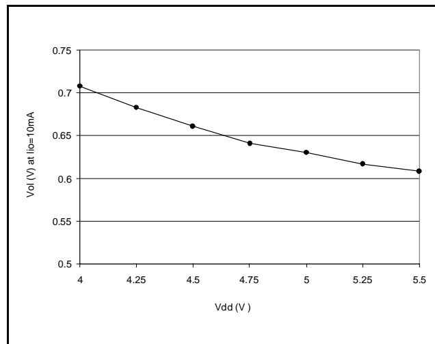
Figure 69. Typical V_{OL} vs. V_{DD} (high-sink I/Os)
