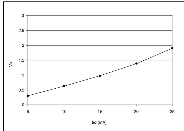
Figure 65. Typical V_{OL} at V_{DD}=5V (high-sink)
