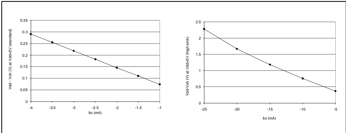
Figure 67. Typical V_{DD}-V_{OH} at V_{DD}=5V
