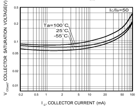
Fig.8 Collector-emitter saturation voltage vs. collector current (II)
