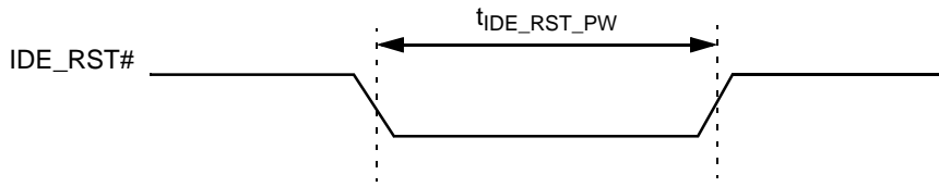
Figure 8-23. IDE Reset Timing Diagram
