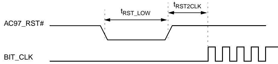
Figure 8-47. AC97 Reset Timing Diagram
