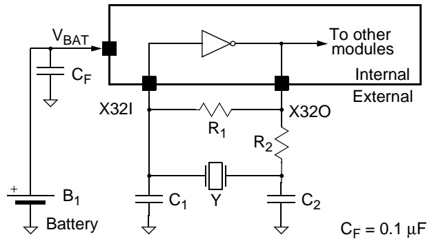
Figure 4-5. Recommended Oscillator External Circuitry
