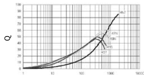
Typical Q vs. Frequency
