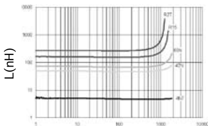
Typical L vs. Frequency
