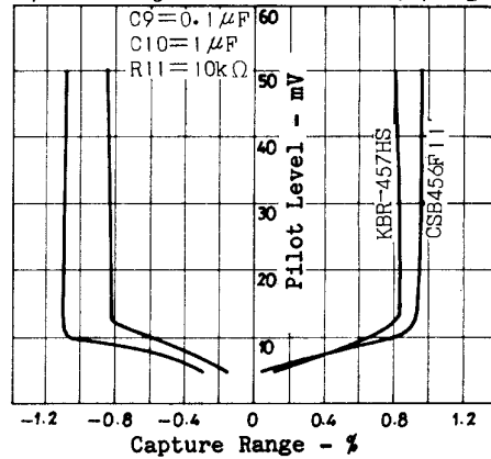
Capture Range Characteristic (3) Fig. 3
