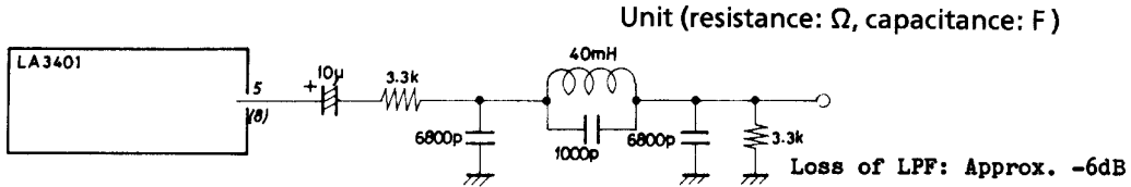
Fig. 16 Sample LC filter circuit (including de-emphasis circuit)
