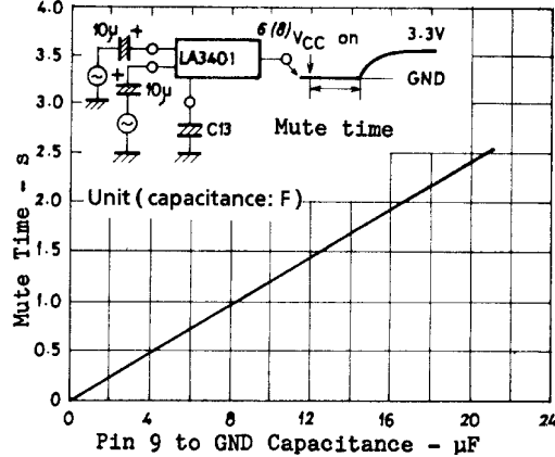
Mute Time - Pin 9 to GND Capacitance Fig. 12
