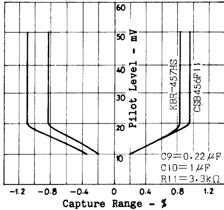
Capture Range Characteristic (2) Fig. 2
