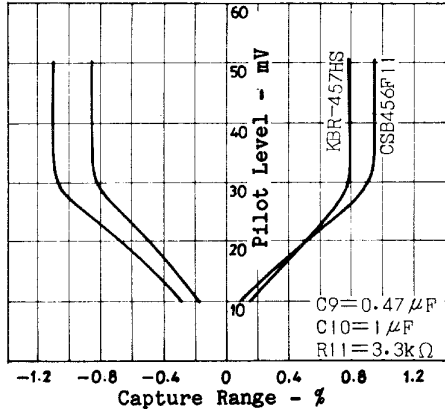
Capture Range Characteristic (4) Fig. 4
