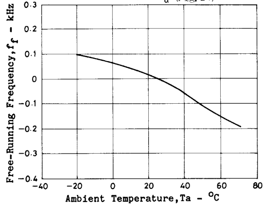
Free-Running Frequency, f_f - T_a (Fig. 24)
