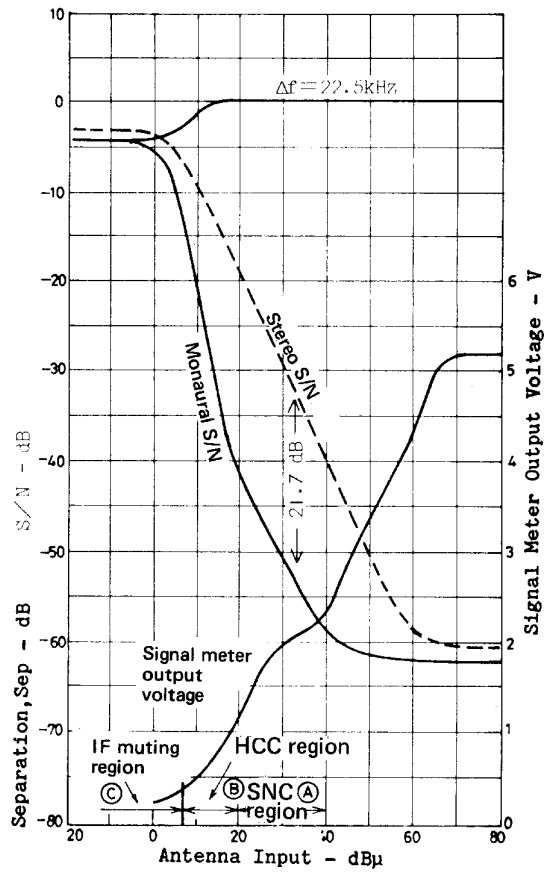
SNC and HCC Operating Regions (Fig.2)
