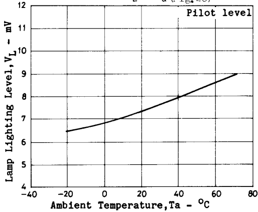
Lamp Lighting Level, V_L - T_a (Fig. 25)
