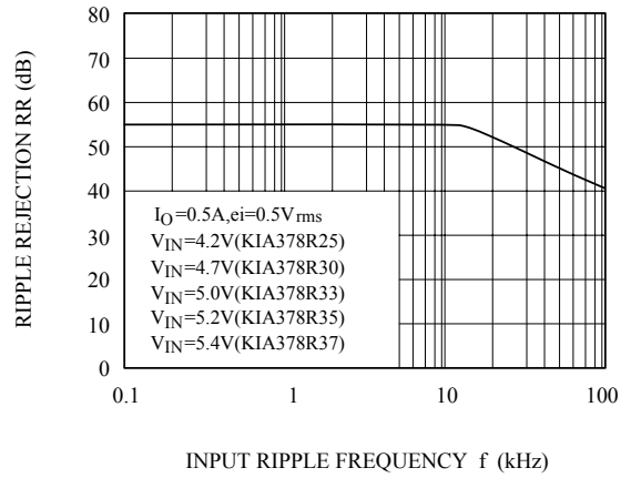
Fig.8-1 f - RR
