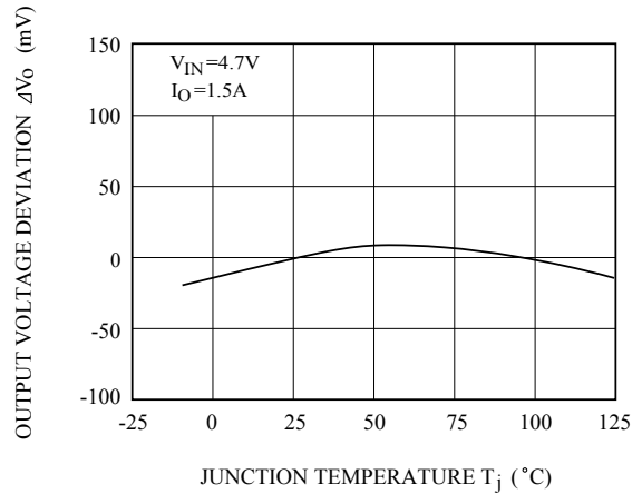
Fig.5-2 T_j - \Delta V_O (KIA378R30)
