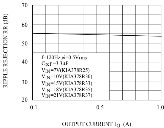
Fig.8-2 I_O - RR
