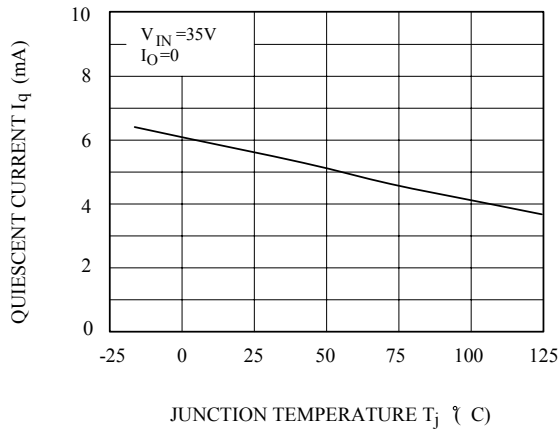
Fig.7 T_j - I_q
