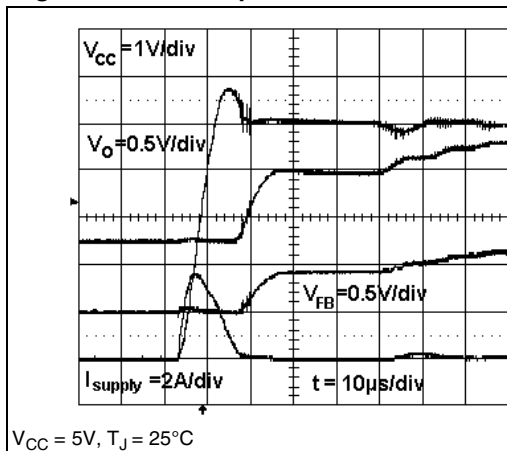
Figure 20. Start-Up transient
