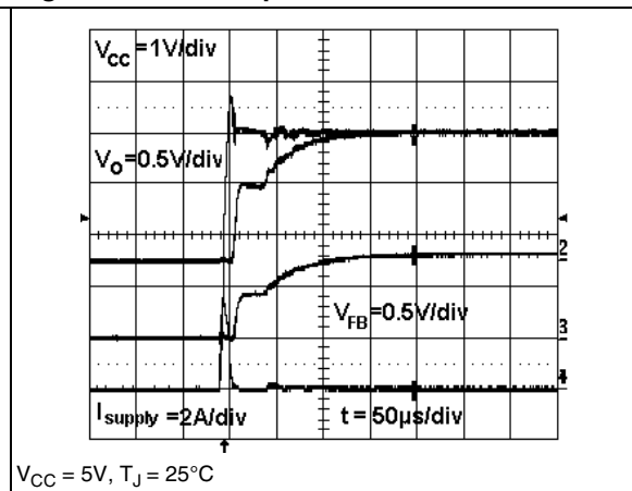
Figure 21. Start-Up transient
