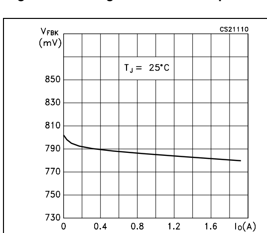
Figure 8. Voltage feedback vs output current
