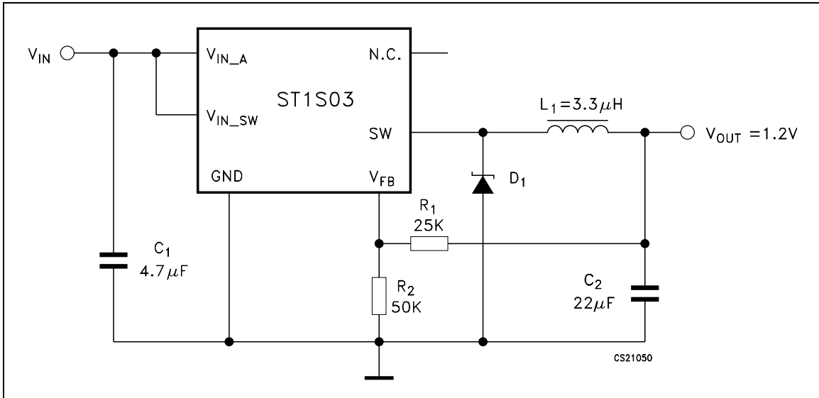
Figure 3. Application circuits
